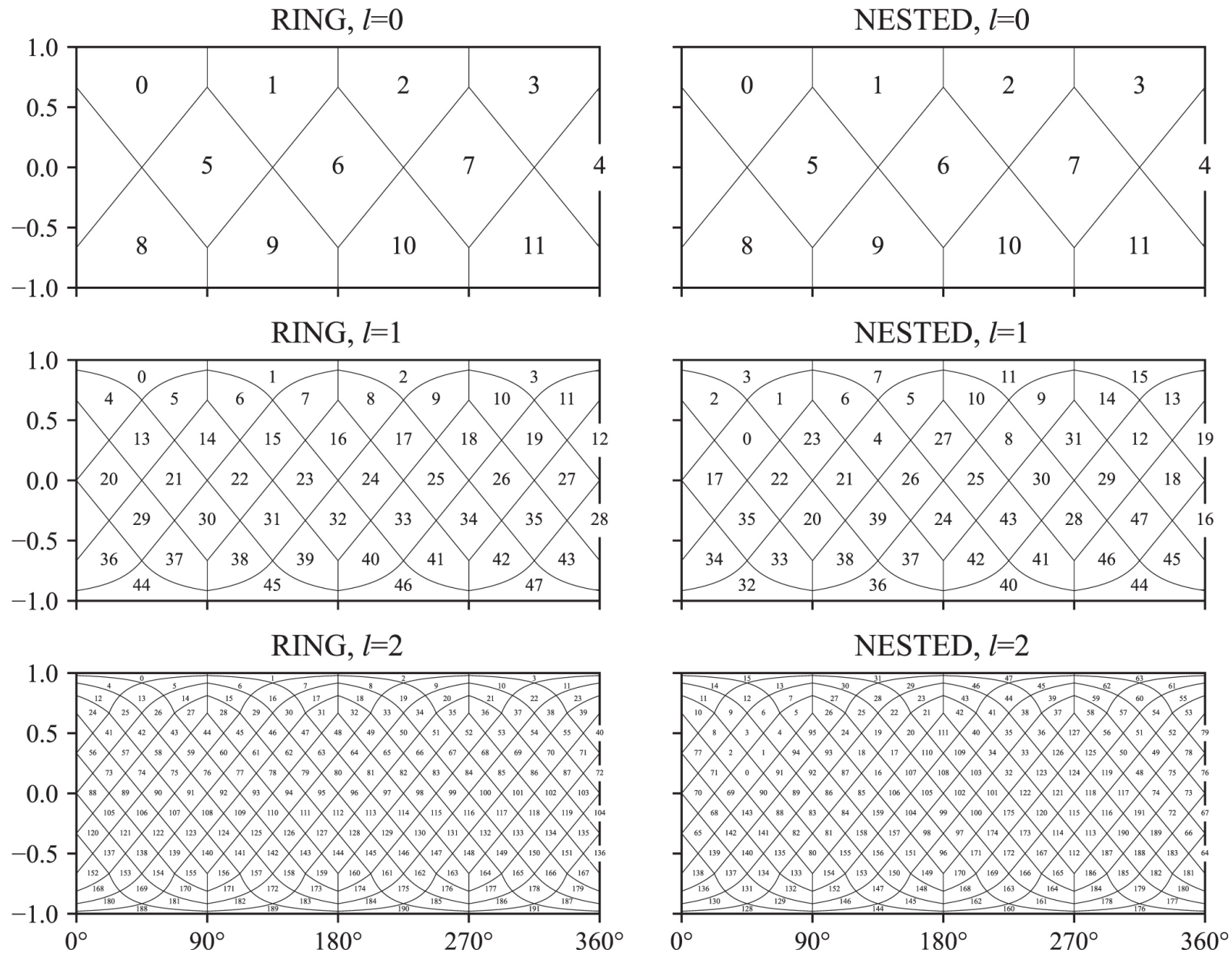
Figure 3. from Leo P. Singer et al 2022 Astron. J. 163 doi:10.3847/1538-3881/ac5ab8 https://dx.doi.org/10.3847/1538-3881/ac5ab8 © 2022. The Author(s). Published by the American Astronomical Society.
