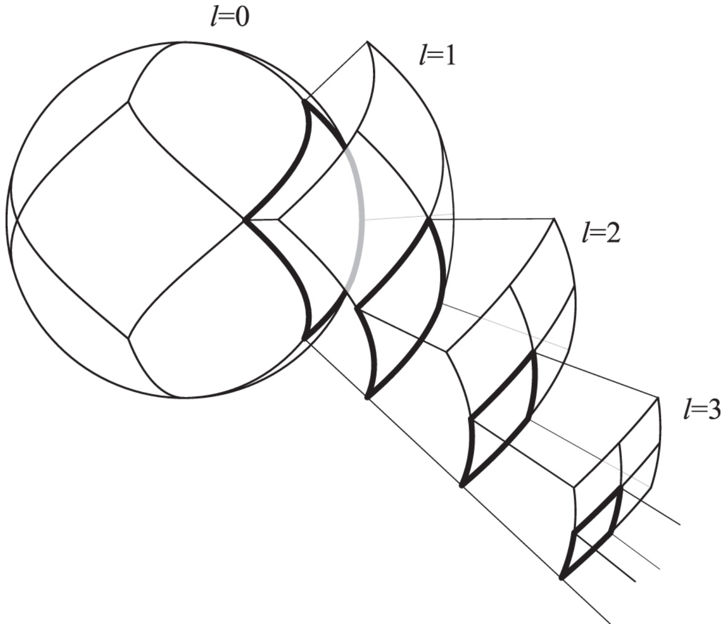
Figure 2. from Leo P. Singer et al 2022 Astron. J. 163 doi:10.3847/1538-3881/ac5ab8 https://dx.doi.org/10.3847/1538-3881/ac5ab8 © 2022. The Author(s). Published by the American Astronomical Society.
