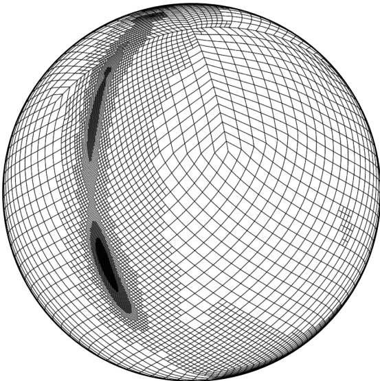
Multi-resolution HEALPix Tiles
