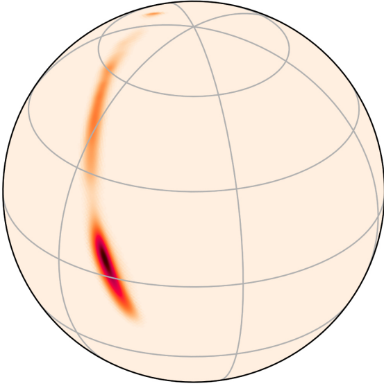
Probability Sky Map
