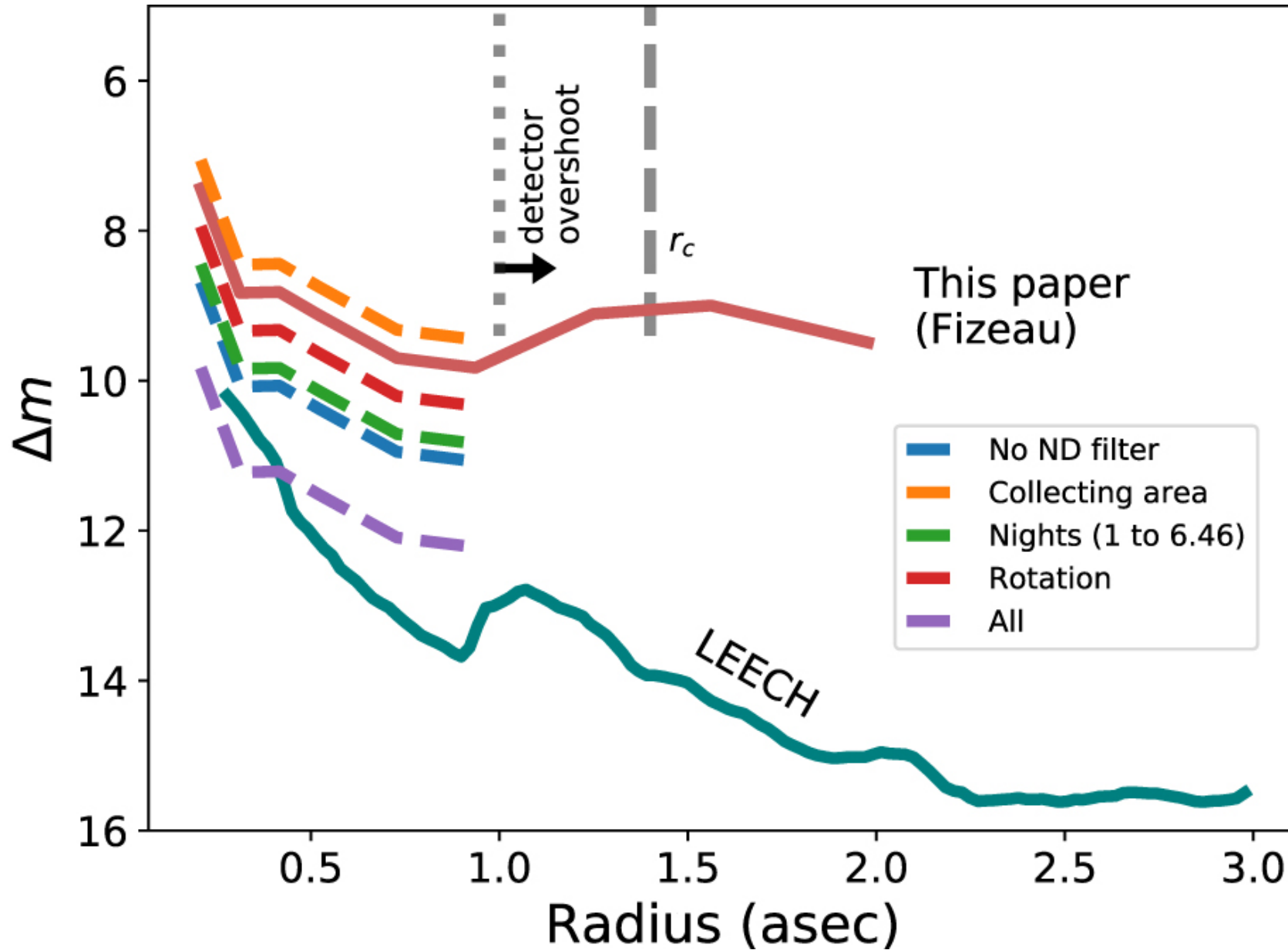
Figure 9. from High-contrast Imaging with Fizeau Interferometry: the Case of Altair null 2022 AJ 163 62 doi:10.3847/1538-3881/ac3b5b http://dx.doi.org/10.3847/1538-3881/ac3b5b © 2022. The Author(s). Published by the American Astronomical Society.
