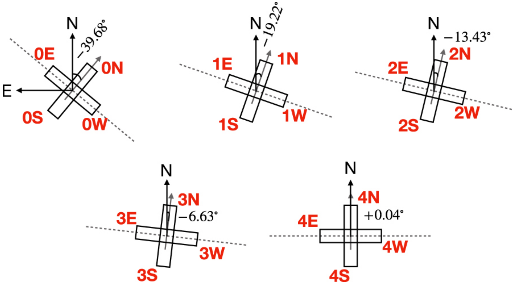
Figure 7. from High-contrast Imaging with Fizeau Interferometry: the Case of Altair null 2022 AJ 163 62 doi:10.3847/1538-3881/ac3b5b http://dx.doi.org/10.3847/1538-3881/ac3b5b © 2022. The Author(s). Published by the American Astronomical Society.
