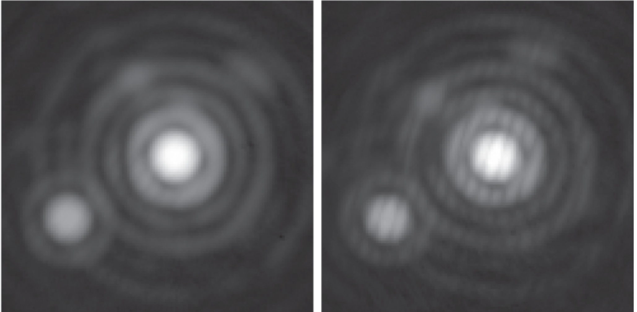
Figure 6. from High-contrast Imaging with Fizeau Interferometry: the Case of Altair null 2022 AJ 163 62 doi:10.3847/1538-3881/ac3b5b http://dx.doi.org/10.3847/1538-3881/ac3b5b © 2022. The Author(s). Published by the American Astronomical Society.
