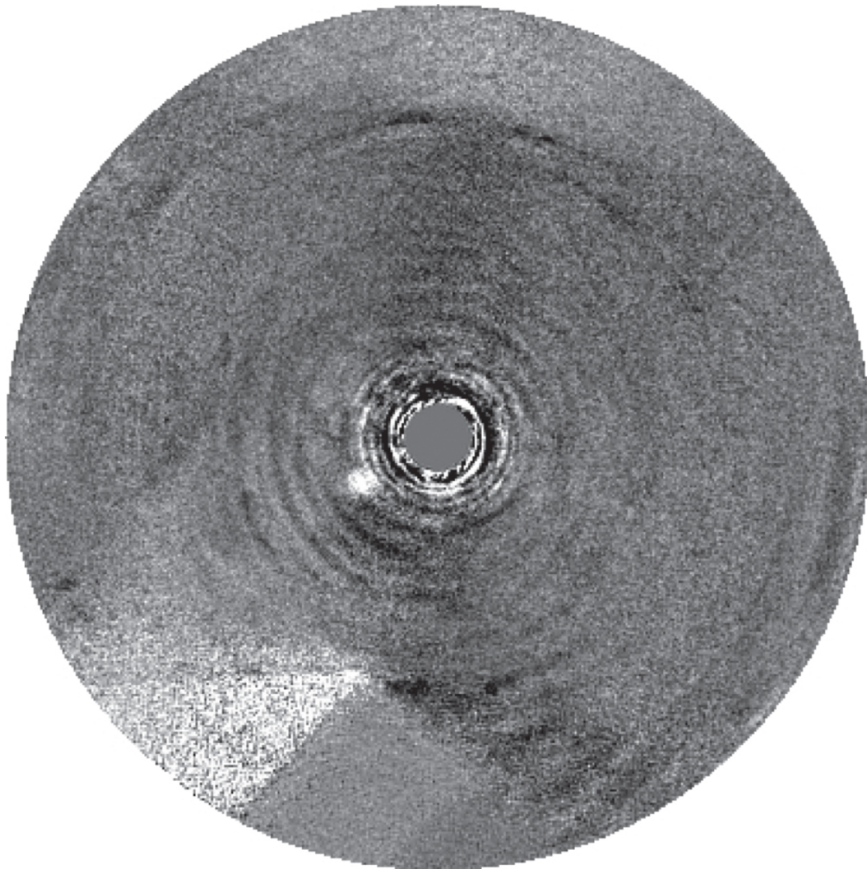
Figure 5. from High-contrast Imaging with Fizeau Interferometry: the Case of Altair null 2022 AJ 163 62 doi:10.3847/1538-3881/ac3b5b http://dx.doi.org/10.3847/1538-3881/ac3b5b © 2022. The Author(s). Published by the American Astronomical Society.
