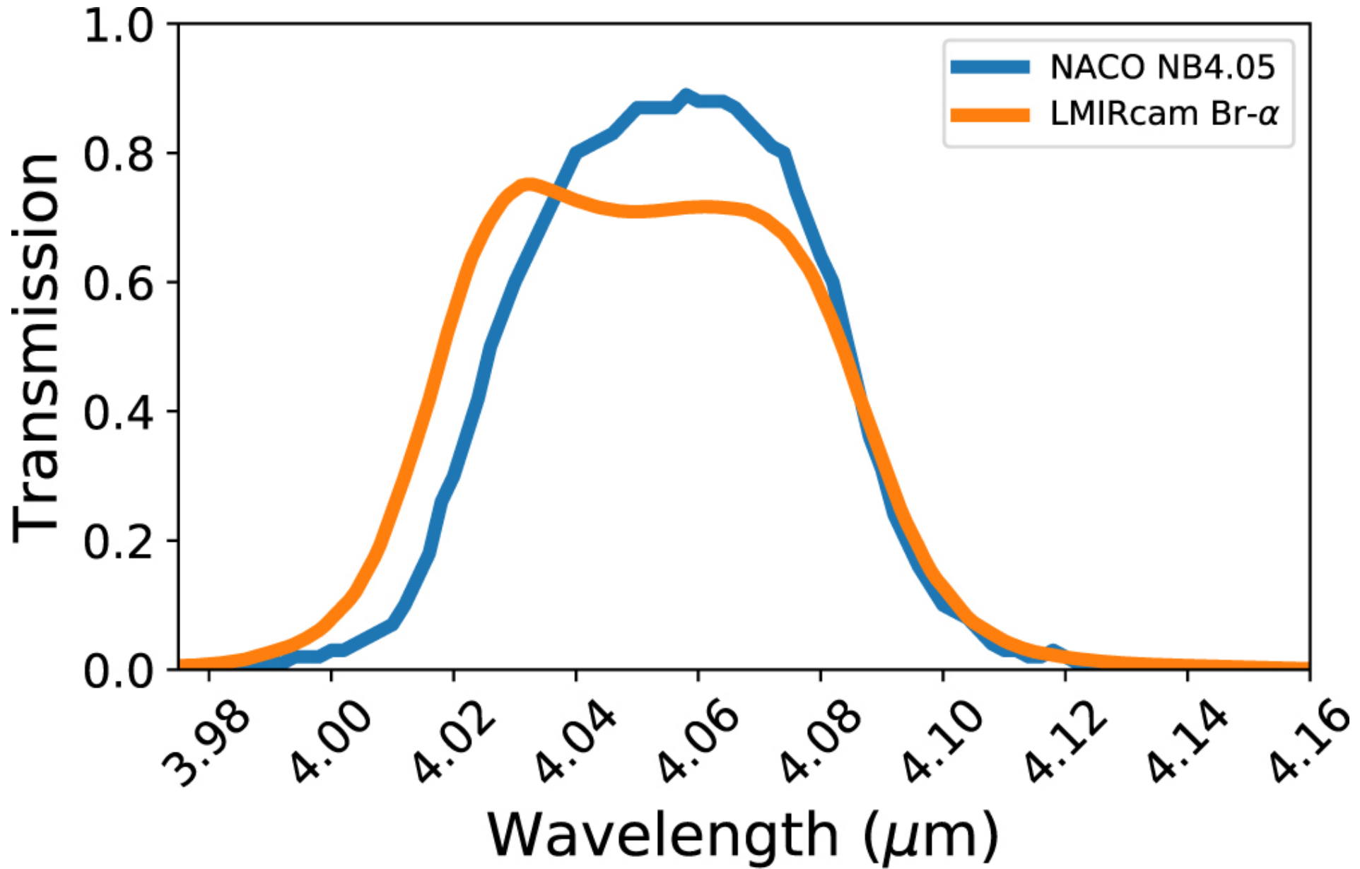
Figure 4. from High-contrast Imaging with Fizeau Interferometry: the Case of Altair null 2022 AJ 163 62 doi:10.3847/1538-3881/ac3b5b http://dx.doi.org/10.3847/1538-3881/ac3b5b © 2022. The Author(s). Published by the American Astronomical Society.
