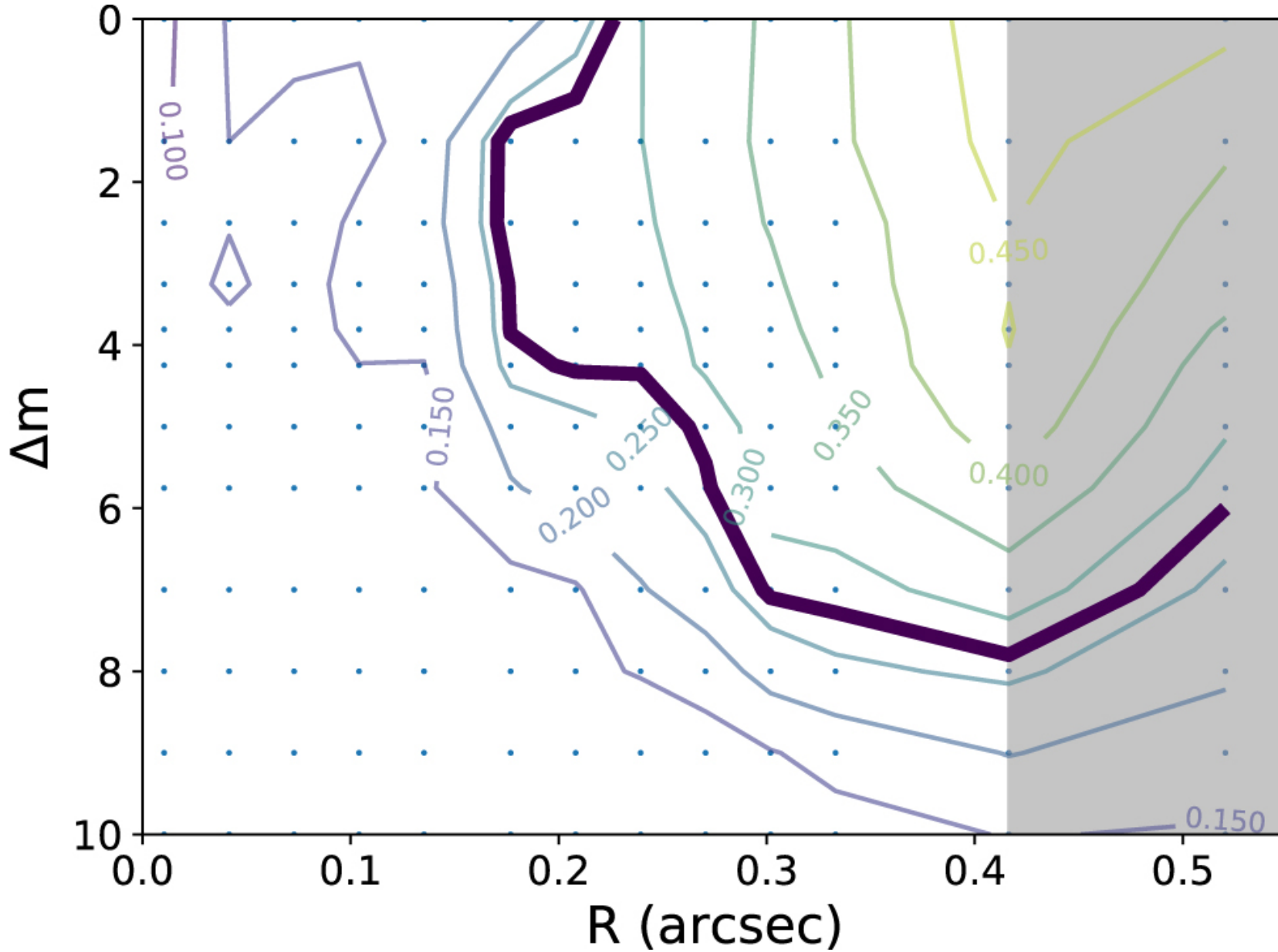
Figure 11. from High-contrast Imaging with Fizeau Interferometry: the Case of Altair null 2022 AJ 163 62 doi:10.3847/1538-3881/ac3b5b http://dx.doi.org/10.3847/1538-3881/ac3b5b © 2022. The Author(s). Published by the American Astronomical Society.
