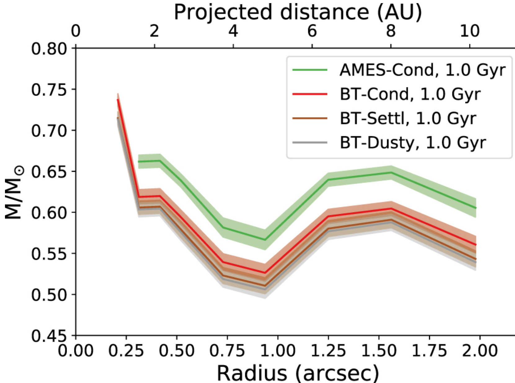
Figure 10. from High-contrast Imaging with Fizeau Interferometry: the Case of Altair null 2022 AJ 163 62 doi:10.3847/1538-3881/ac3b5b http://dx.doi.org/10.3847/1538-3881/ac3b5b © 2022. The Author(s). Published by the American Astronomical Society.
