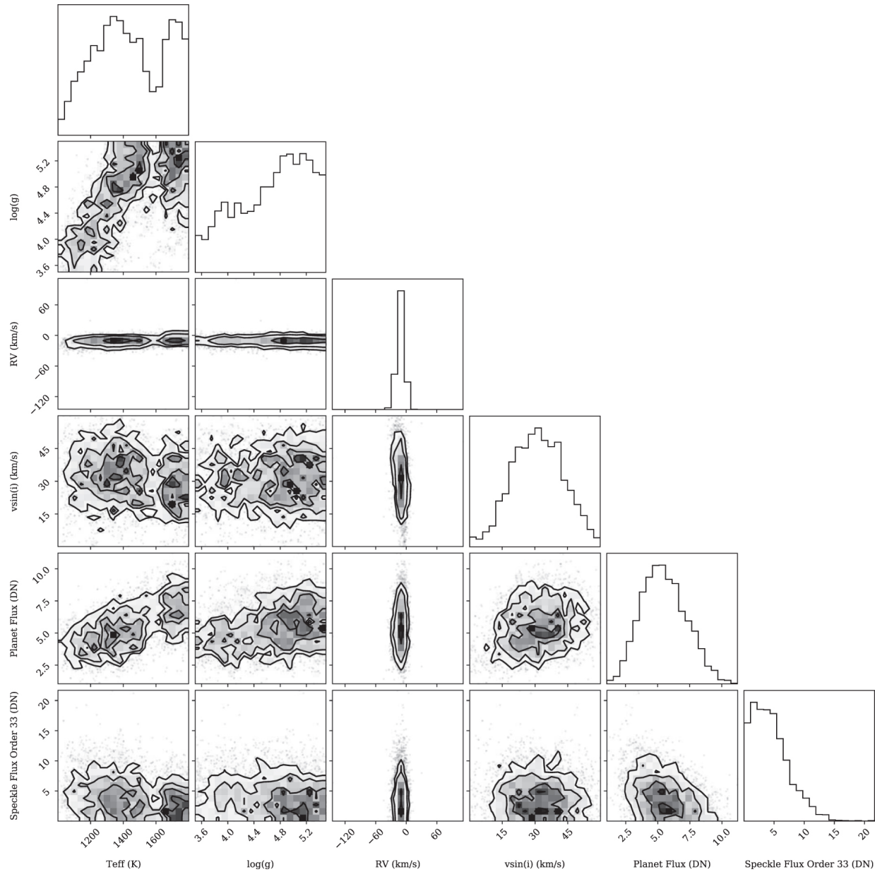
Figure 7. from Detection and Bulk Properties of the HR 8799 Planets with High-resolution Spectroscopy null 2021 AJ 162 148 doi:10.3847/1538-3881/ac1349 https://dx.doi.org/10.3847/1538-3881/ac1349 © 2021. The Author(s). Published by the American Astronomical Society.
