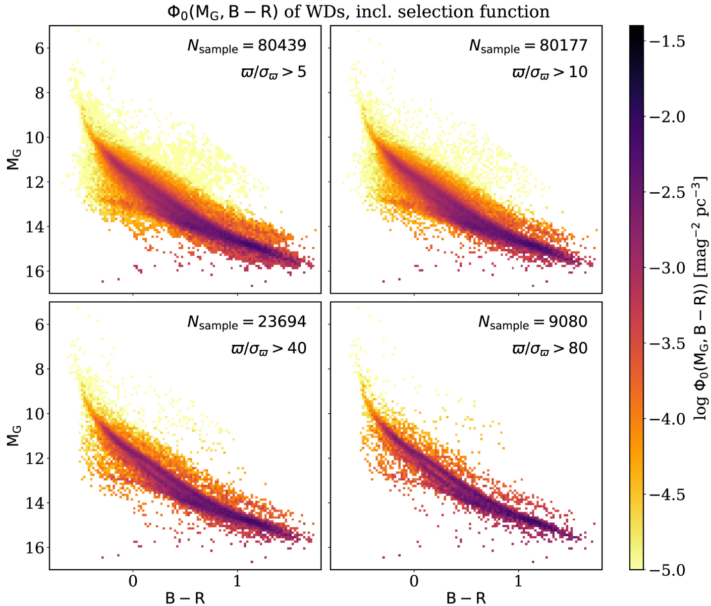
Figure 9. from Selection Functions in Astronomical Data Modeling, with the Space Density of White Dwarfs as a Worked Example null 2021 AJ 162 142 doi:10.3847/1538-3881/ac0c13 https://dx.doi.org/10.3847/1538-3881/ac0c13 © 2021. The Author(s). Published by the American Astronomical Society.
