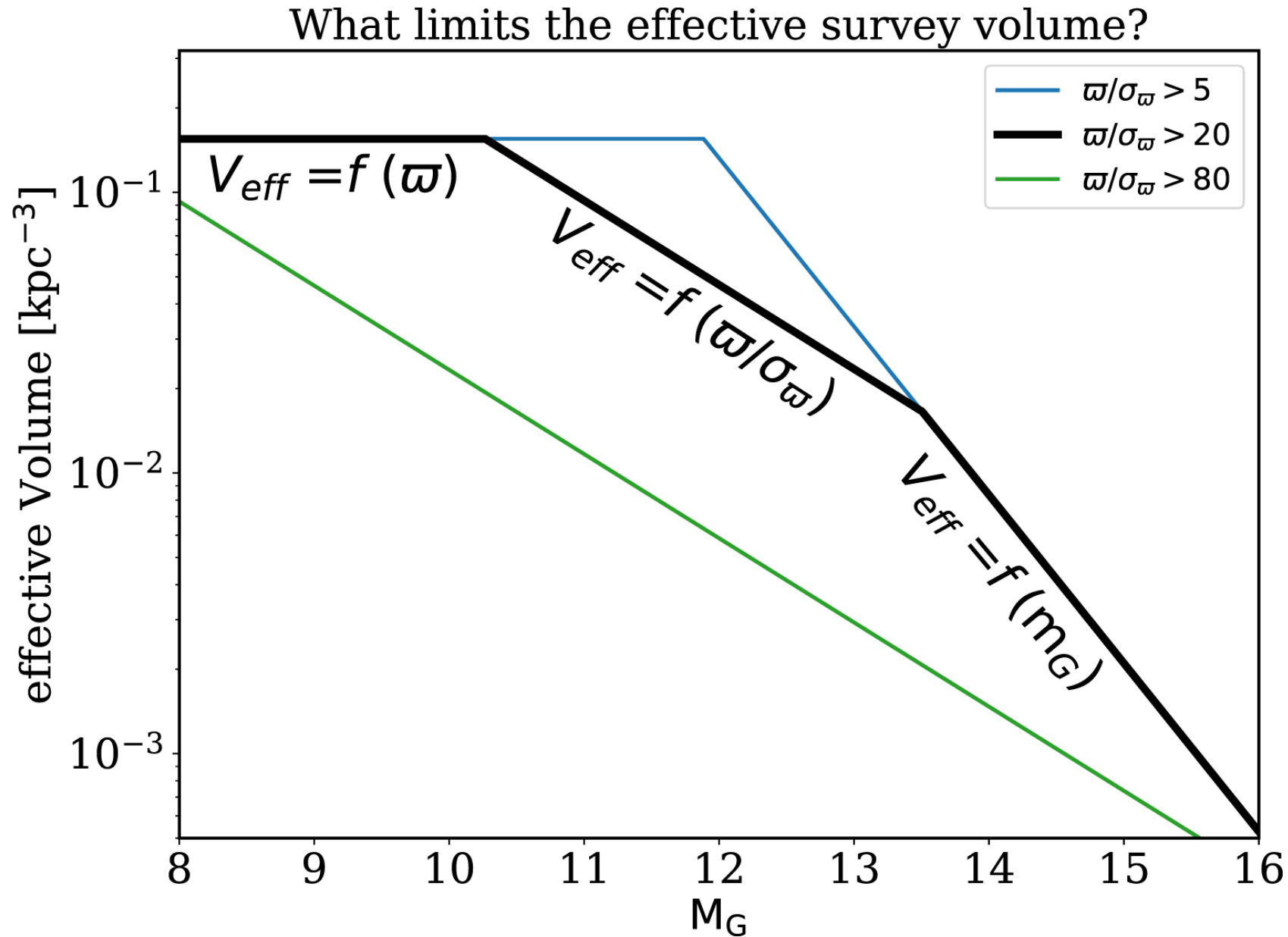
Figure 6. from Selection Functions in Astronomical Data Modeling, with the Space Density of White Dwarfs as a Worked Example null 2021 AJ 162 142 doi:10.3847/1538-3881/ac0c13 https://dx.doi.org/10.3847/1538-3881/ac0c13 © 2021. The Author(s). Published by the American Astronomical Society.
