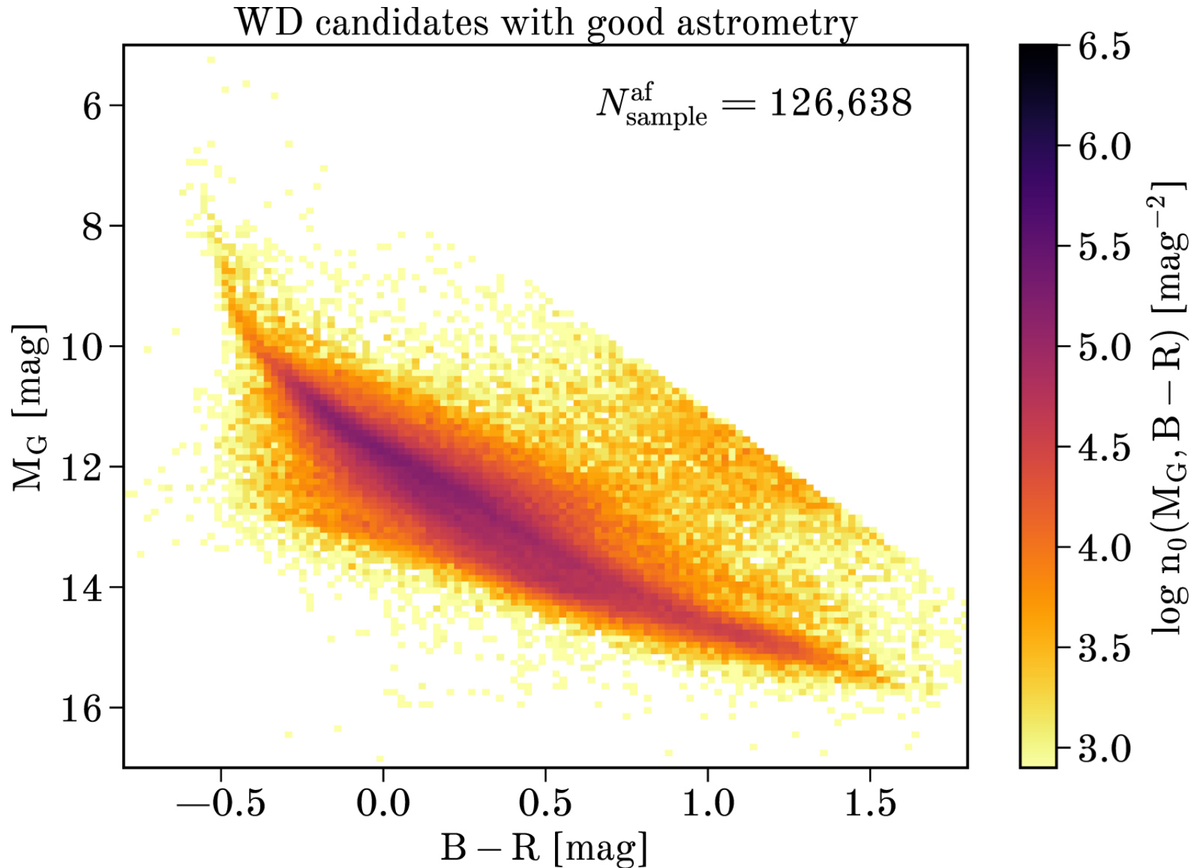
Figure 3. from Selection Functions in Astronomical Data Modeling, with the Space Density of White Dwarfs as a Worked Example null 2021 AJ 162 142 doi:10.3847/1538-3881/ac0c13 http://dx.doi.org/10.3847/1538-3881/ac0c13 © 2021. The Author(s). Published by the American Astronomical Society.
