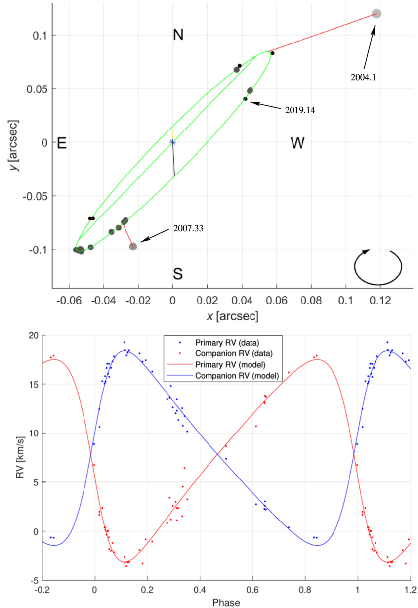
Figure 5. from Orbits and Masses of Binaries from Speckle Interferometry at SOAR null 2021 AJ 161 155 doi:10.3847/1538-3881/abdb28 https://dx.doi.org/10.3847/1538-3881/abdb28 © 2021. The American Astronomical Society. All rights reserved.
