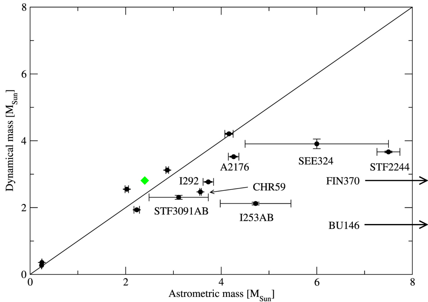
Figure 4. from Orbits and Masses of Binaries from Speckle Interferometry at SOAR null 2021 AJ 161 155 doi:10.3847/1538-3881/abdb28 https://dx.doi.org/10.3847/1538-3881/abdb28 © 2021. The American Astronomical Society. All rights reserved.
