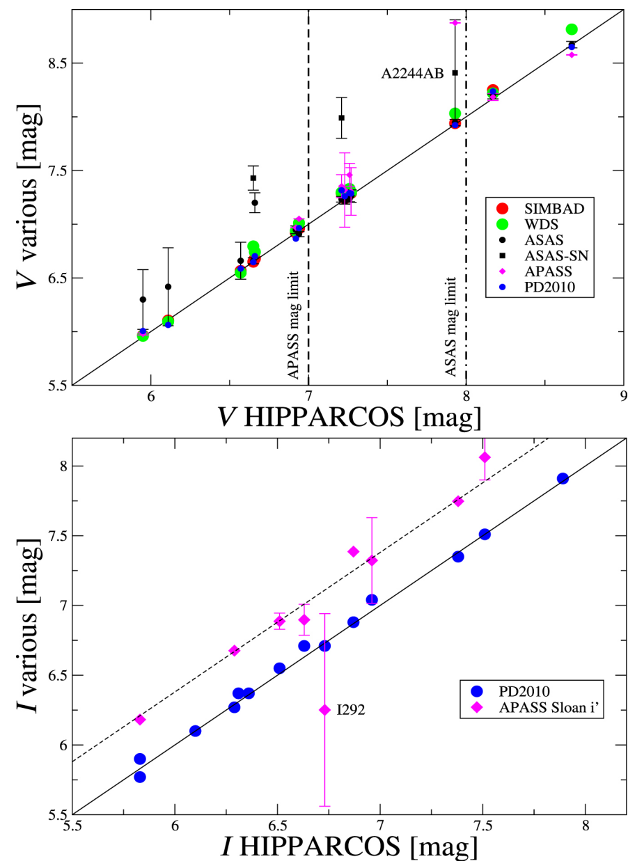
Figure 1. from Orbits and Masses of Binaries from Speckle Interferometry at SOAR null 2021 AJ 161 155 doi:10.3847/1538-3881/abdb28 https://dx.doi.org/10.3847/1538-3881/abdb28 © 2021. The American Astronomical Society. All rights reserved.
