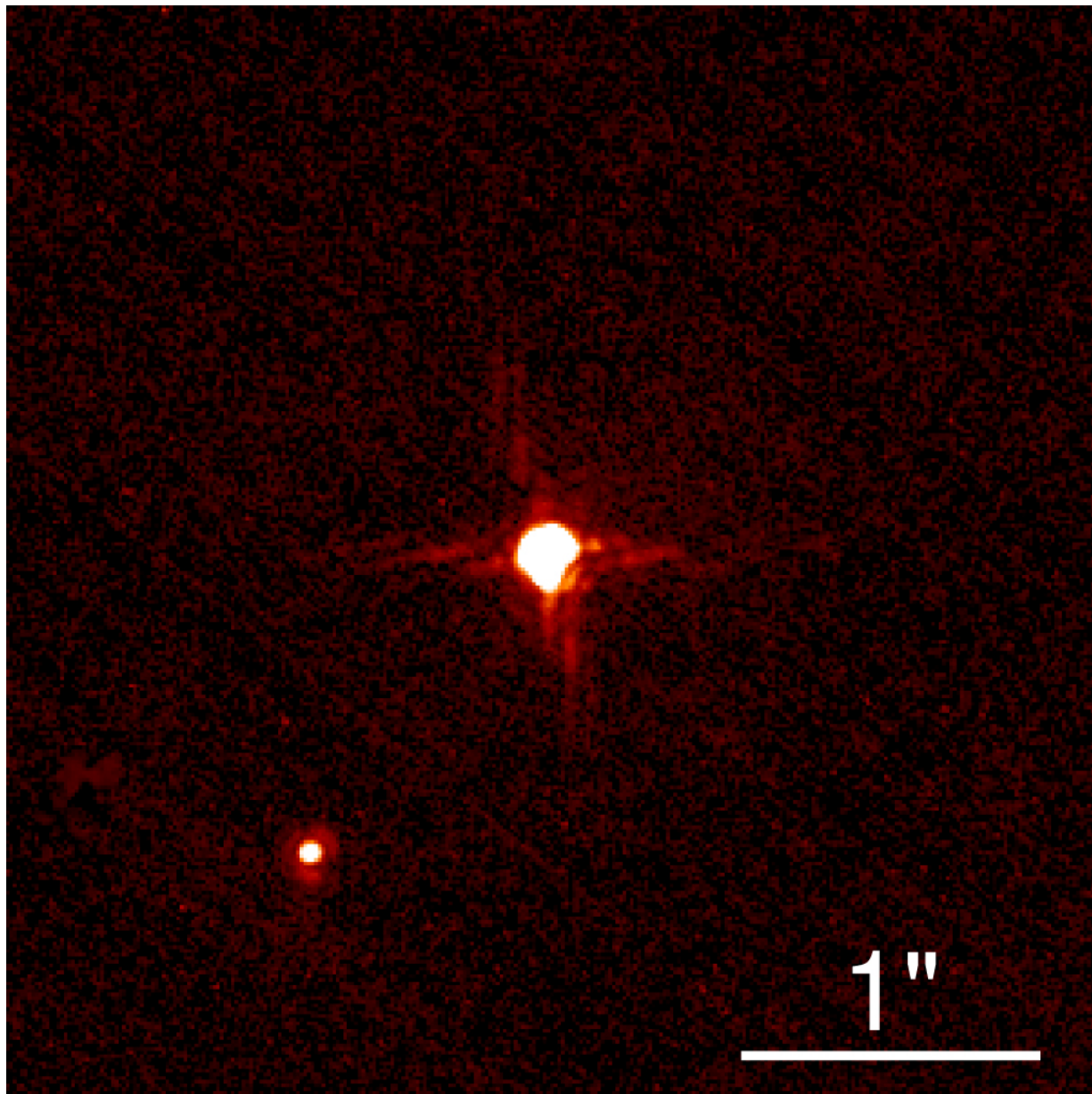
Figure 9. from Three New Late-type Stellar Companions to Very Dusty WISE Debris Disks Identified with SPHERE Imaging null 2021 AJ 161 78 doi:10.3847/1538-3881/abcfca https://dx.doi.org/10.3847/1538-3881/abcfca © 2021. The American Astronomical Society. All rights reserved.
