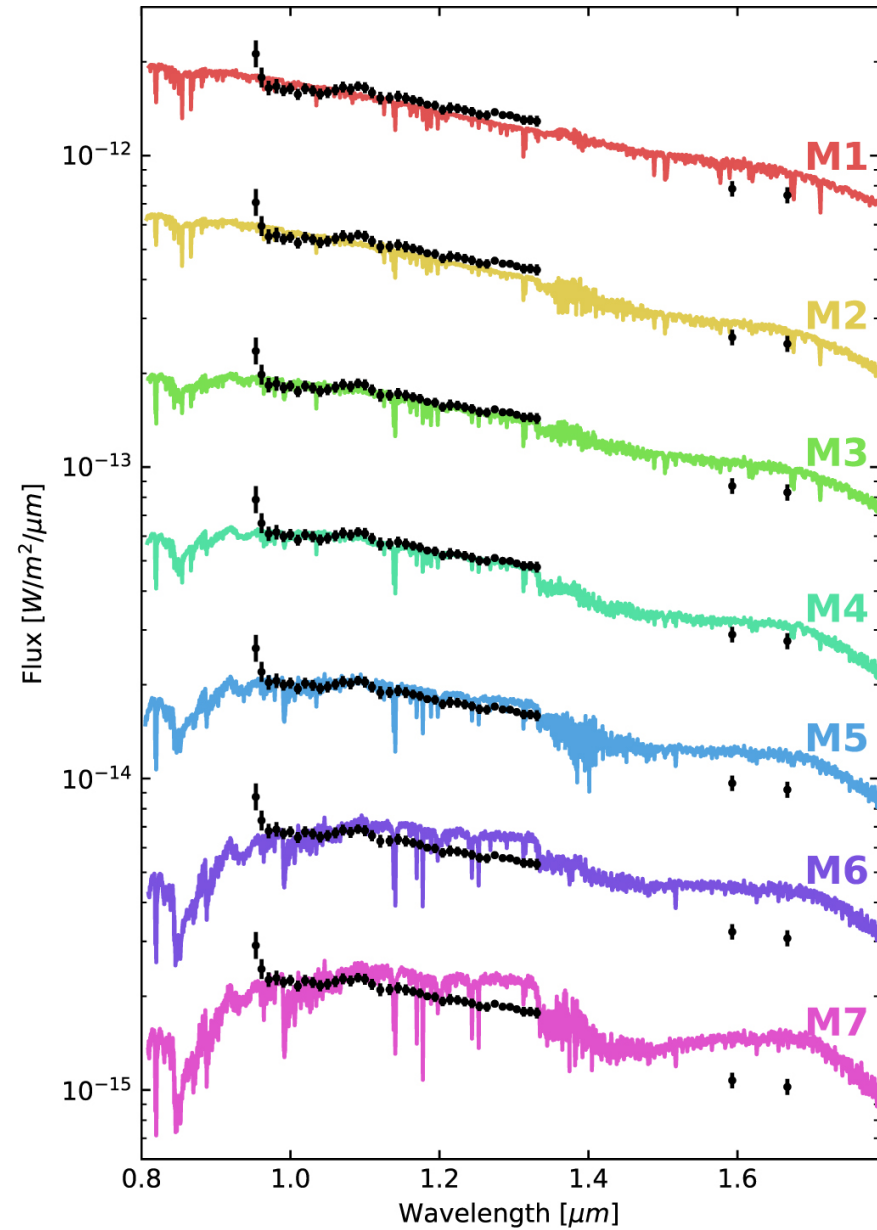
Figure 8. from Three New Late-type Stellar Companions to Very Dusty WISE Debris Disks Identified with SPHERE Imaging null 2021 AJ 161 78 doi:10.3847/1538-3881/abcfca https://dx.doi.org/10.3847/1538-3881/abcfca © 2021. The American Astronomical Society. All rights reserved.
