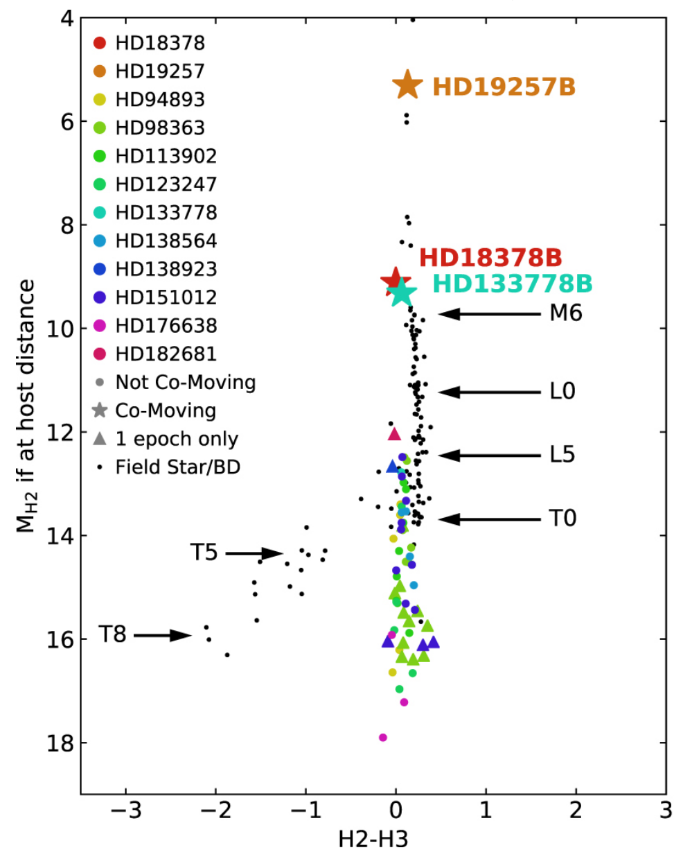
Figure 6. from Three New Late-type Stellar Companions to Very Dusty WISE Debris Disks Identified with SPHERE Imaging null 2021 AJ 161 78 doi:10.3847/1538-3881/abcfca https://dx.doi.org/10.3847/1538-3881/abcfca © 2021. The American Astronomical Society. All rights reserved.
