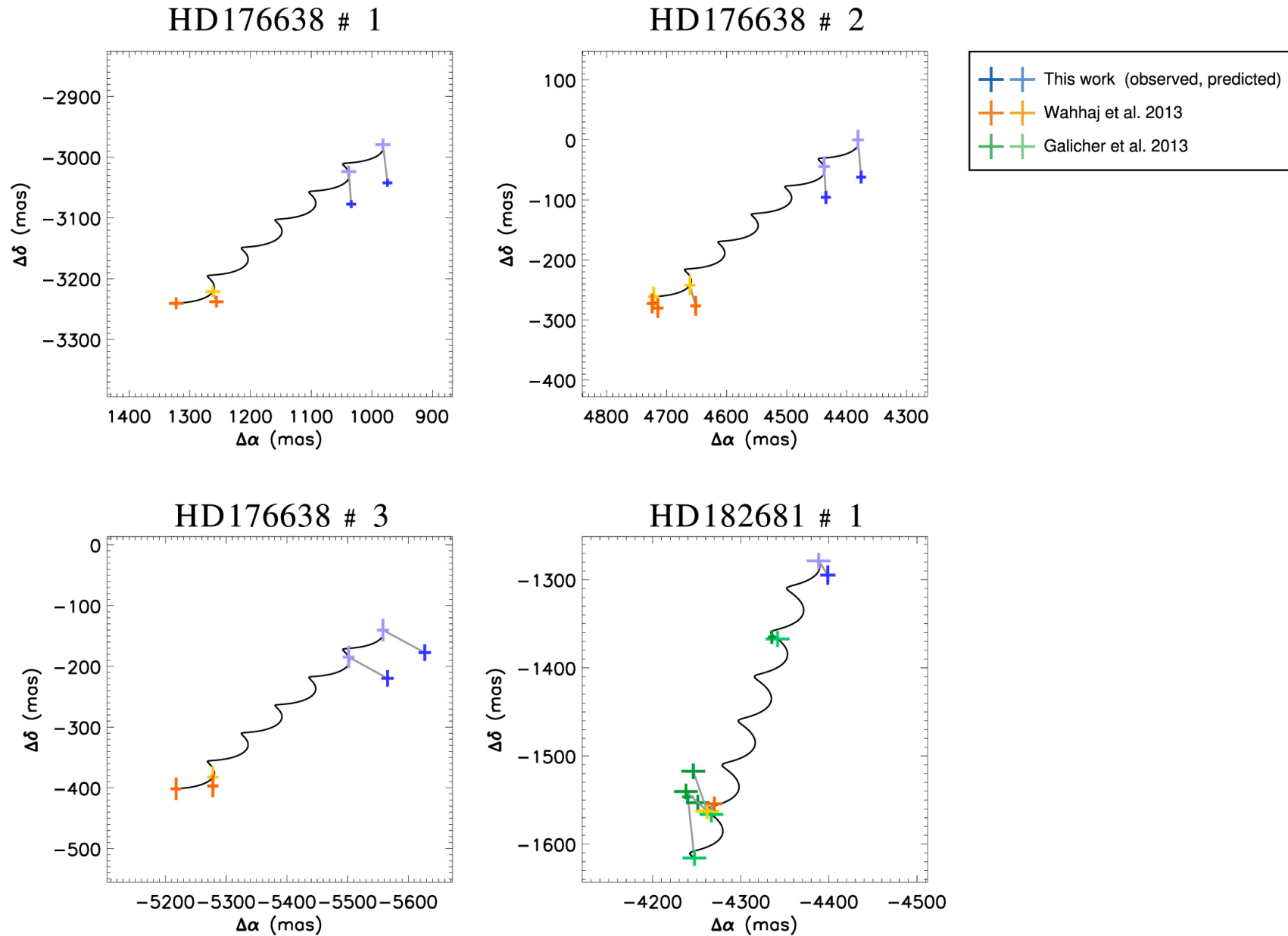
Figure 5. from Three New Late-type Stellar Companions to Very Dusty WISE Debris Disks Identified with SPHERE Imaging null 2021 AJ 161 78 doi:10.3847/1538-3881/abcfca https://dx.doi.org/10.3847/1538-3881/abcfca © 2021. The American Astronomical Society. All rights reserved.
