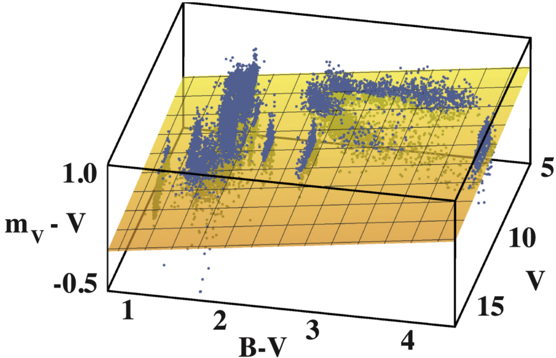
Figure 6. from The Relationship between Photometric Measurements and Visual Magnitude Estimates for Red Stars null 2021 AJ 161 75 doi:10.3847/1538-3881/abcd9c https://dx.doi.org/10.3847/1538-3881/abcd9c © 2021. The American Astronomical Society. All rights reserved.
