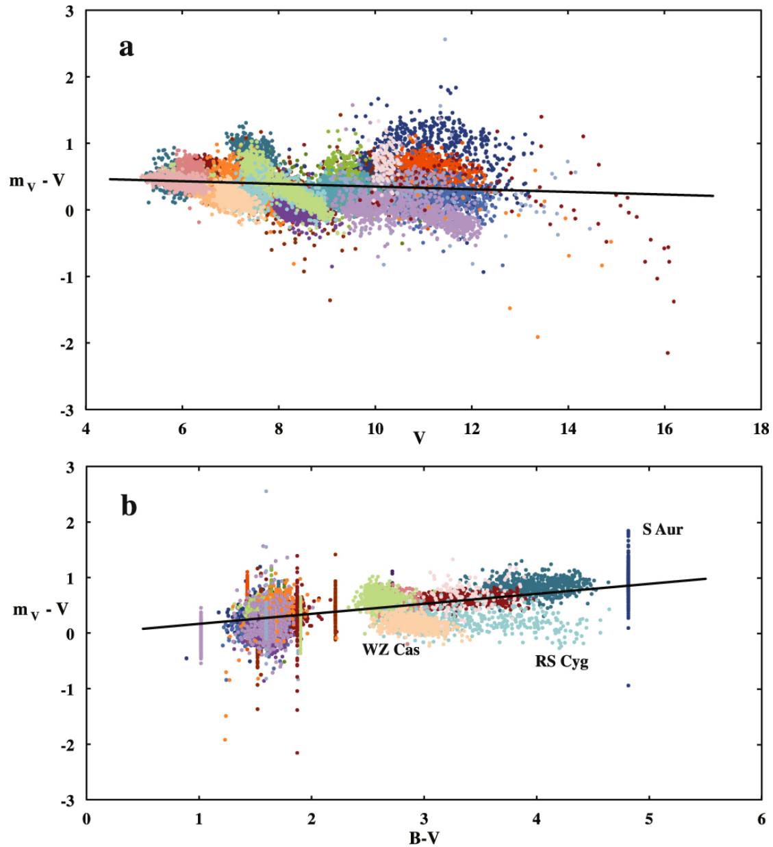
Figure 4. from The Relationship between Photometric Measurements and Visual Magnitude Estimates for Red Stars null 2021 AJ 161 75 doi:10.3847/1538-3881/abcd9c https://dx.doi.org/10.3847/1538-3881/abcd9c © 2021. The American Astronomical Society. All rights reserved.
