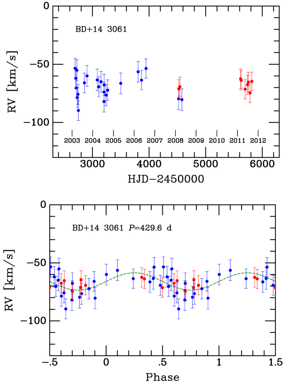
Figure 6. from BD+14°3061: A Luminous Yellow Post-AGB Star in the Galactic Halo null 2020 AJ 160 274 doi:10.3847/1538-3881/abc177 http://dx.doi.org/10.3847/1538-3881/abc177 © 2020. The American Astronomical Society. All rights reserved.
