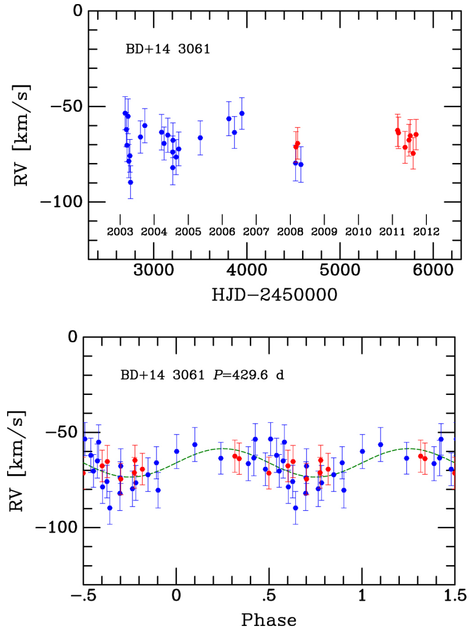
Figure 6. from BD+14°3061: A Luminous Yellow Post-AGB Star in the Galactic Halo null 2020 AJ 160 274 doi:10.3847/1538-3881/abc177 https://dx.doi.org/10.3847/1538-3881/abc177 © 2020. The American Astronomical Society. All rights reserved.
