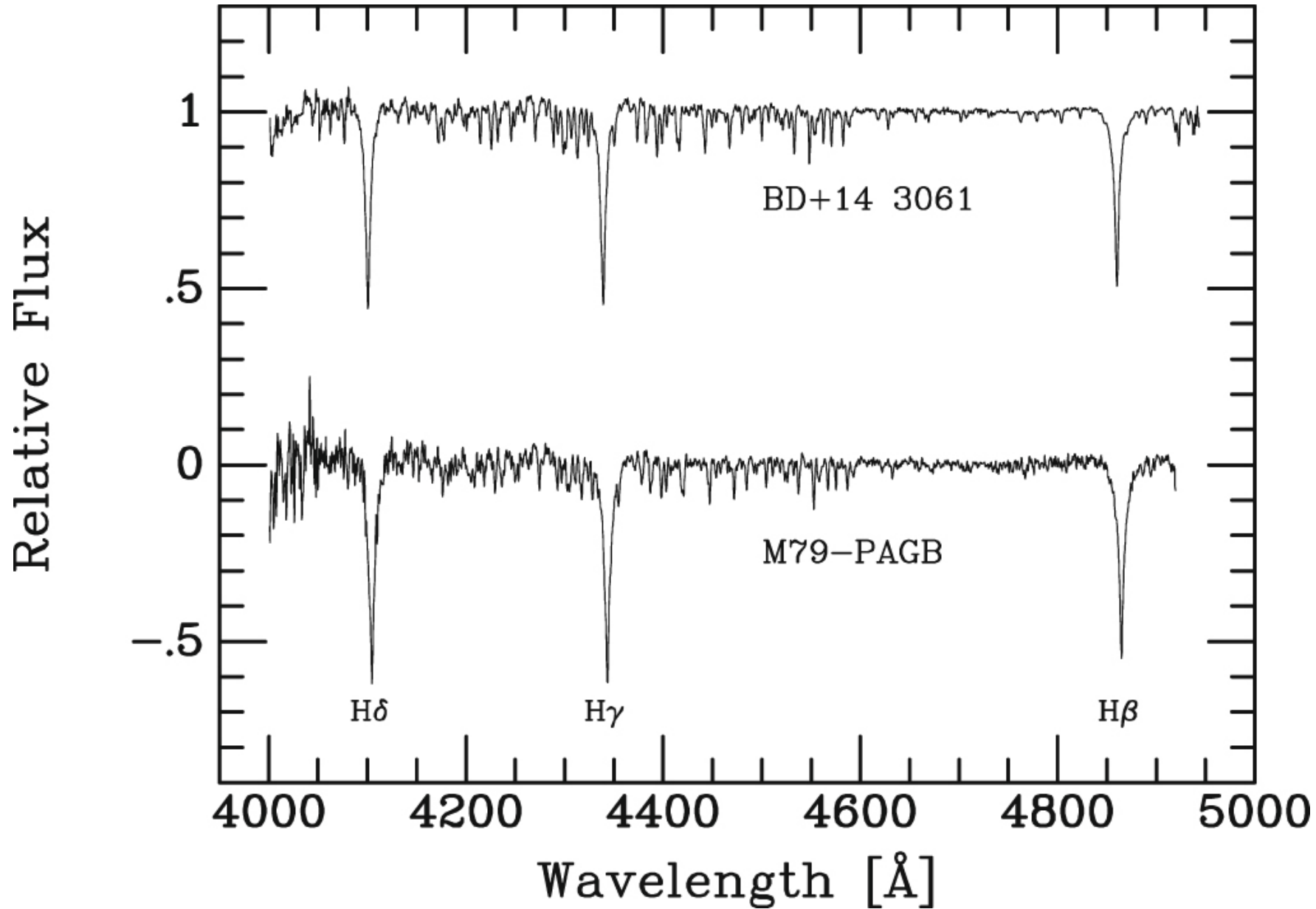
Figure 5. from BD+14°3061: A Luminous Yellow Post-AGB Star in the Galactic Halo null 2020 AJ 160 274 doi:10.3847/1538-3881/abc177 http://dx.doi.org/10.3847/1538-3881/abc177 © 2020. The American Astronomical Society. All rights reserved.
