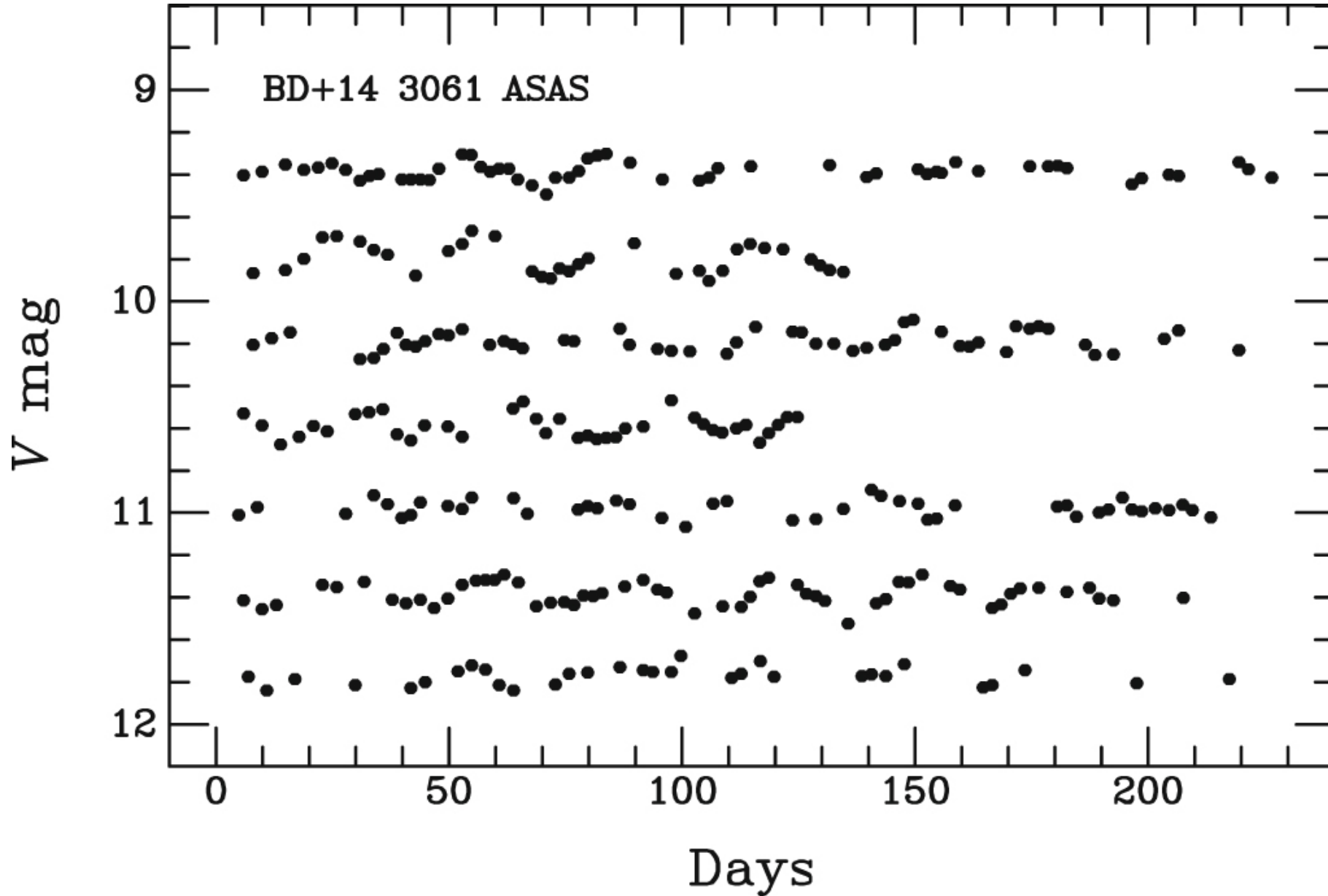
Figure 4. from BD+14°3061: A Luminous Yellow Post-AGB Star in the Galactic Halo null 2020 AJ 160 274 doi:10.3847/1538-3881/abc177 http://dx.doi.org/10.3847/1538-3881/abc177 © 2020. The American Astronomical Society. All rights reserved.
