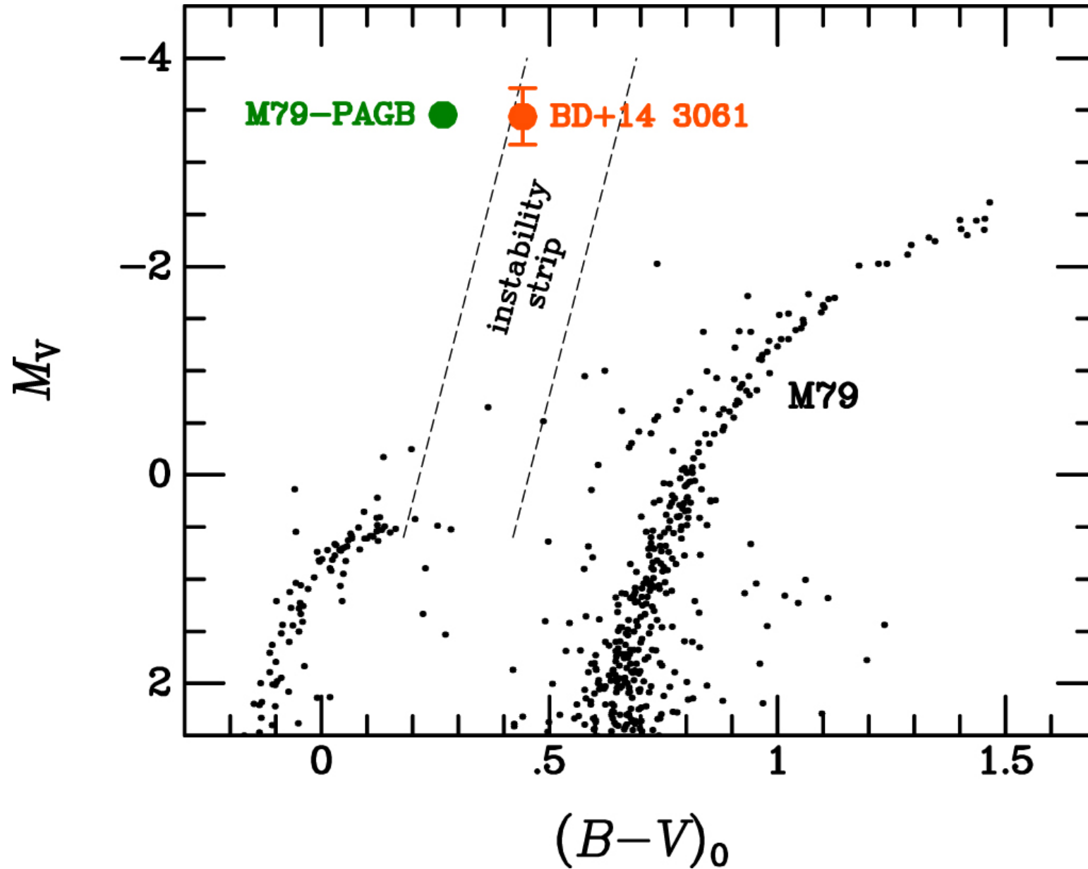
Figure 2. from BD+14°3061: A Luminous Yellow Post-AGB Star in the Galactic Halo null 2020 AJ 160 274 doi:10.3847/1538-3881/abc177 https://dx.doi.org/10.3847/1538-3881/abc177 © 2020. The American Astronomical Society. All rights reserved.
