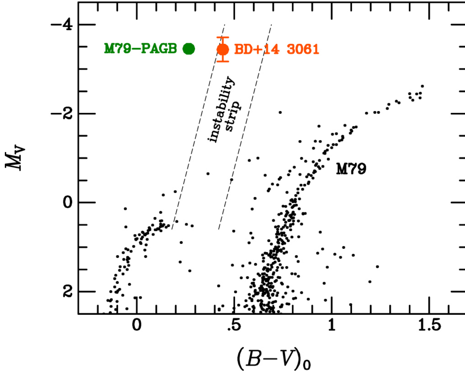
Figure 2. from BD+14°3061: A Luminous Yellow Post-AGB Star in the Galactic Halo null 2020 AJ 160 274 doi:10.3847/1538-3881/abc177 http://dx.doi.org/10.3847/1538-3881/abc177 © 2020. The American Astronomical Society. All rights reserved.
