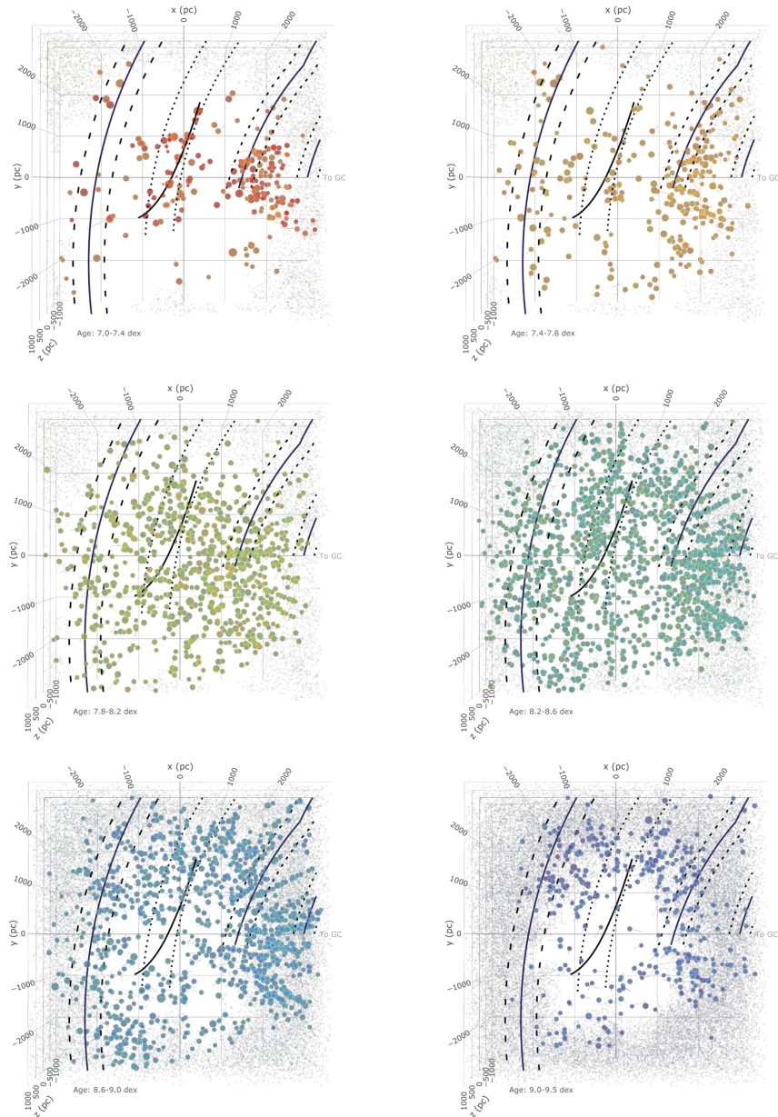
Figure 7. from Untangling the Galaxy. II. Structure within 3 kpc null 2020 AJ 160 279 doi:10.3847/1538-3881/abc0e6 https://dx.doi.org/10.3847/1538-3881/abc0e6 © 2020. The American Astronomical Society. All rights reserved.
