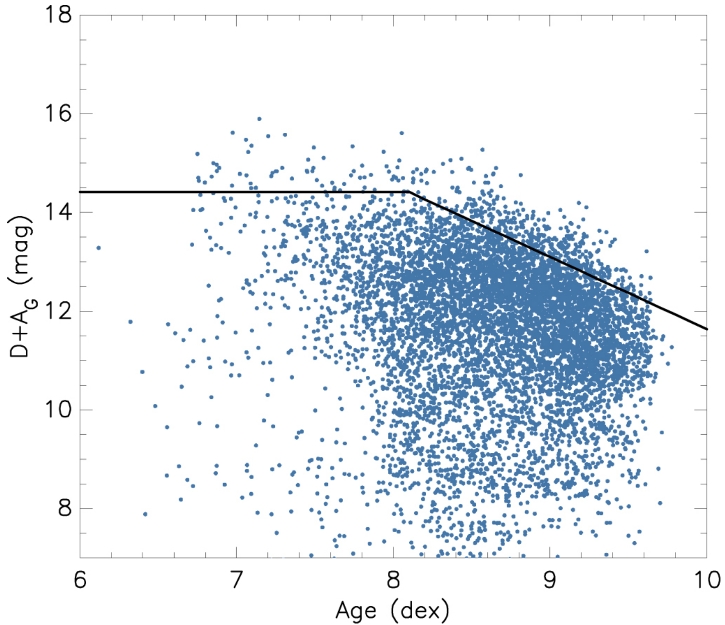
Figure 5. from Untangling the Galaxy. II. Structure within 3 kpc null 2020 AJ 160 279 doi:10.3847/1538-3881/abc0e6 https://dx.doi.org/10.3847/1538-3881/abc0e6 © 2020. The American Astronomical Society. All rights reserved.
