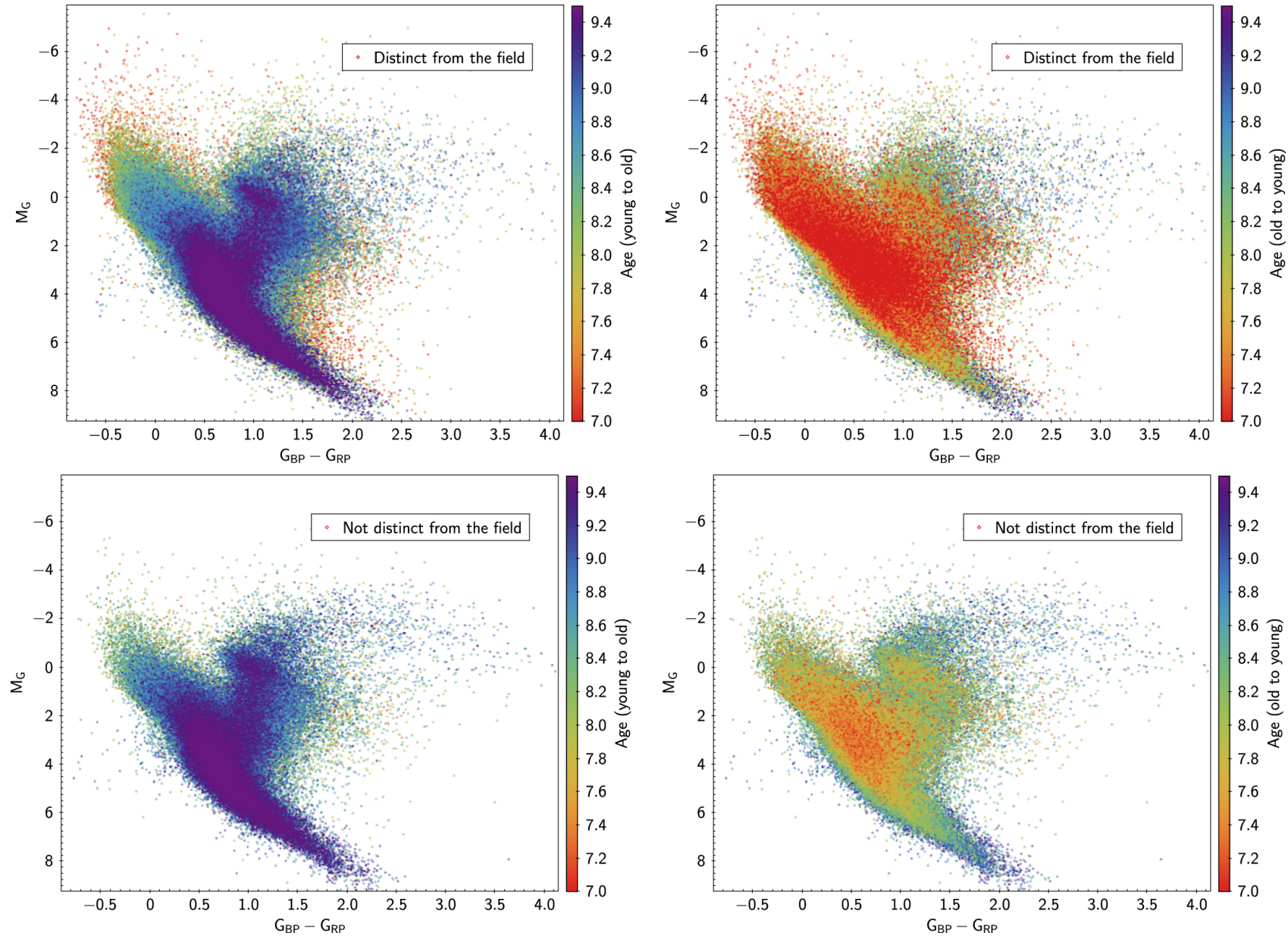
Figure 4. from Untangling the Galaxy. II. Structure within 3 kpc null 2020 AJ 160 279 doi:10.3847/1538-3881/abc0e6 https://dx.doi.org/10.3847/1538-3881/abc0e6 © 2020. The American Astronomical Society. All rights reserved.
