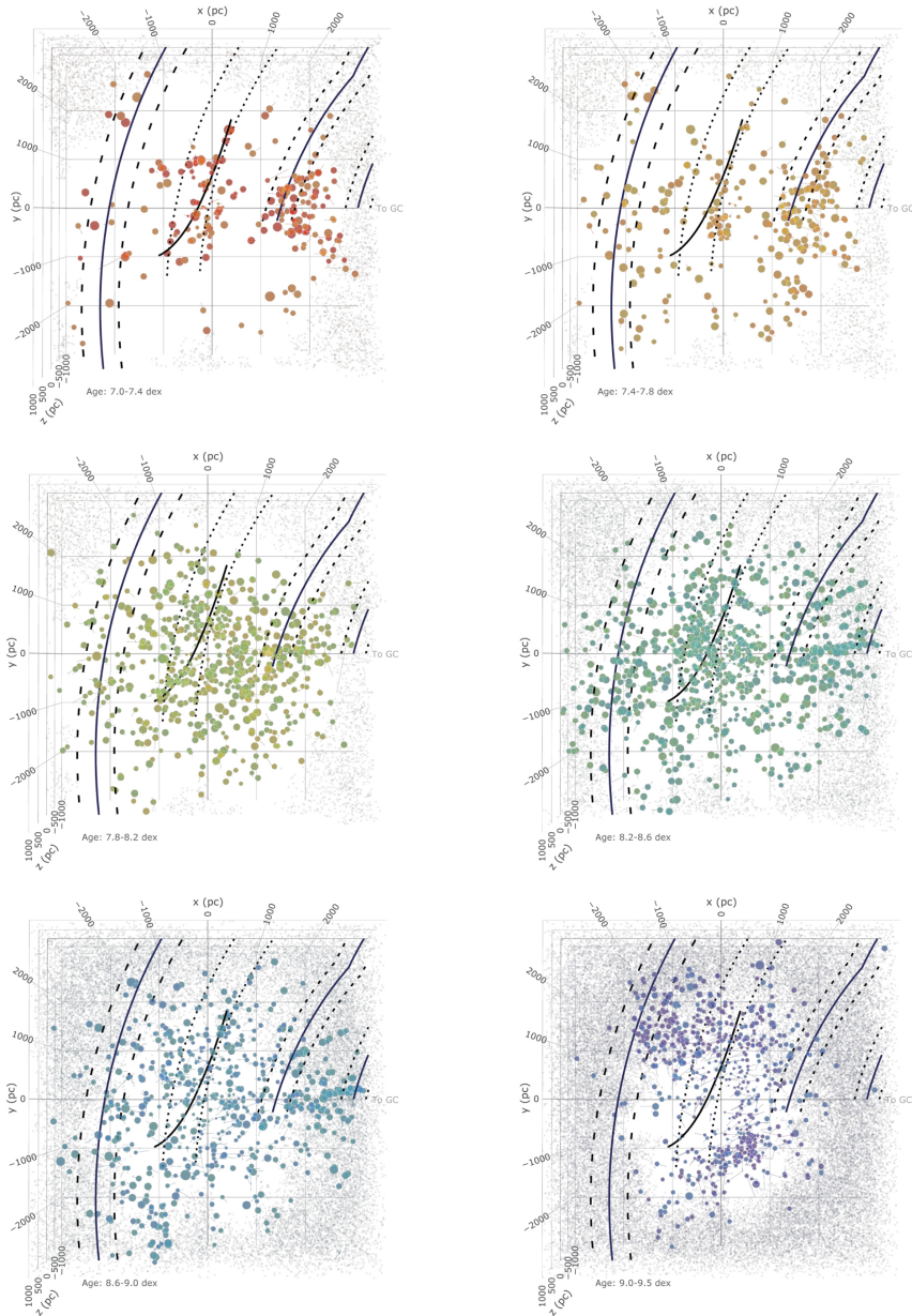
Figure 3. from Untangling the Galaxy. II. Structure within 3 kpc null 2020 AJ 160 279 doi:10.3847/1538-3881/abc0e6 https://dx.doi.org/10.3847/1538-3881/abc0e6 © 2020. The American Astronomical Society. All rights reserved.
