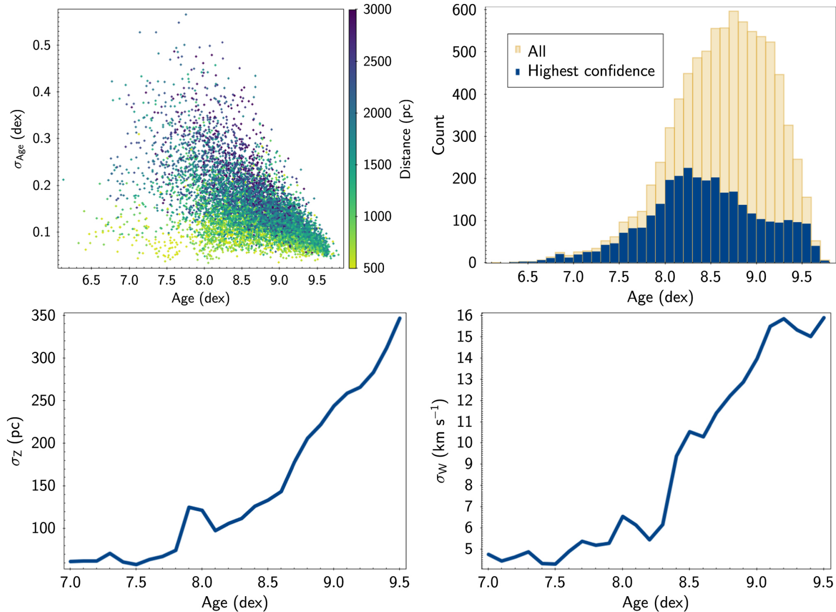
Figure 2. from Untangling the Galaxy. II. Structure within 3 kpc null 2020 AJ 160 279 doi:10.3847/1538-3881/abc0e6 https://dx.doi.org/10.3847/1538-3881/abc0e6 © 2020. The American Astronomical Society. All rights reserved.
