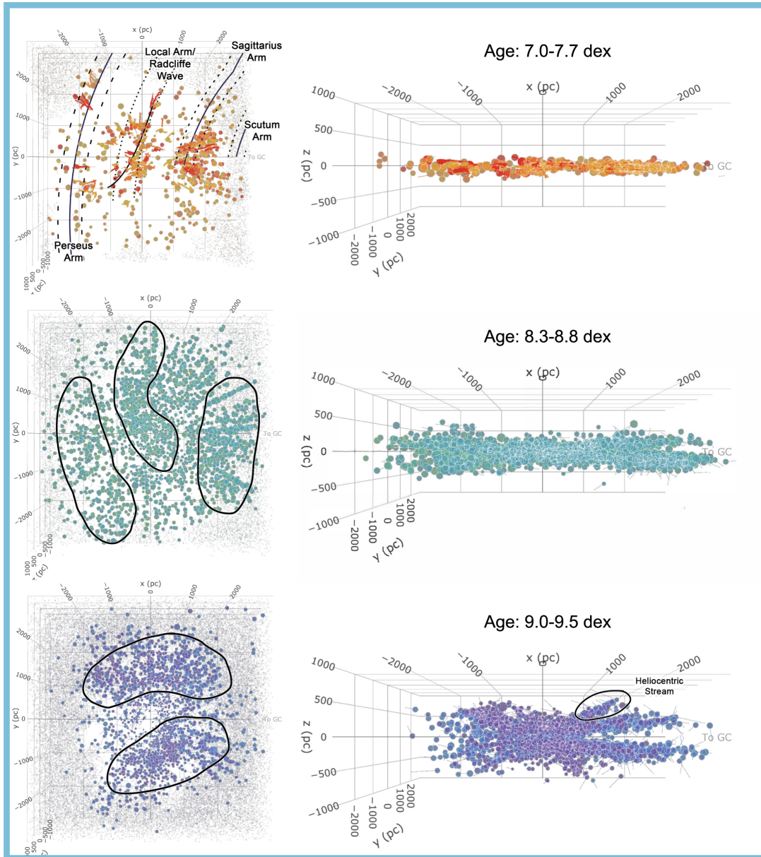
Figure 1. from Untangling the Galaxy. II. Structure within 3 kpc null 2020 AJ 160 279 doi:10.3847/1538-3881/abc0e6 https://dx.doi.org/10.3847/1538-3881/abc0e6 © 2020. The American Astronomical Society. All rights reserved.
