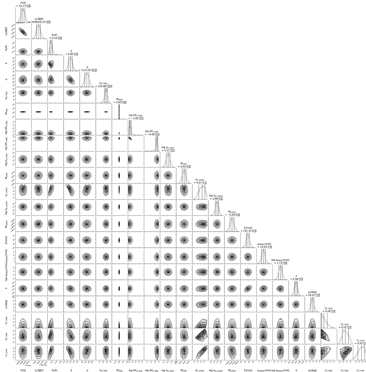
Figure 8. from A Highly Eccentric Warm Jupiter Orbiting TIC 237913194 null 2020 AJ 160 275 doi:10.3847/1538-3881/abbe03 https://dx.doi.org/10.3847/1538-3881/abbe03 © 2020. The American Astronomical Society. All rights reserved.
