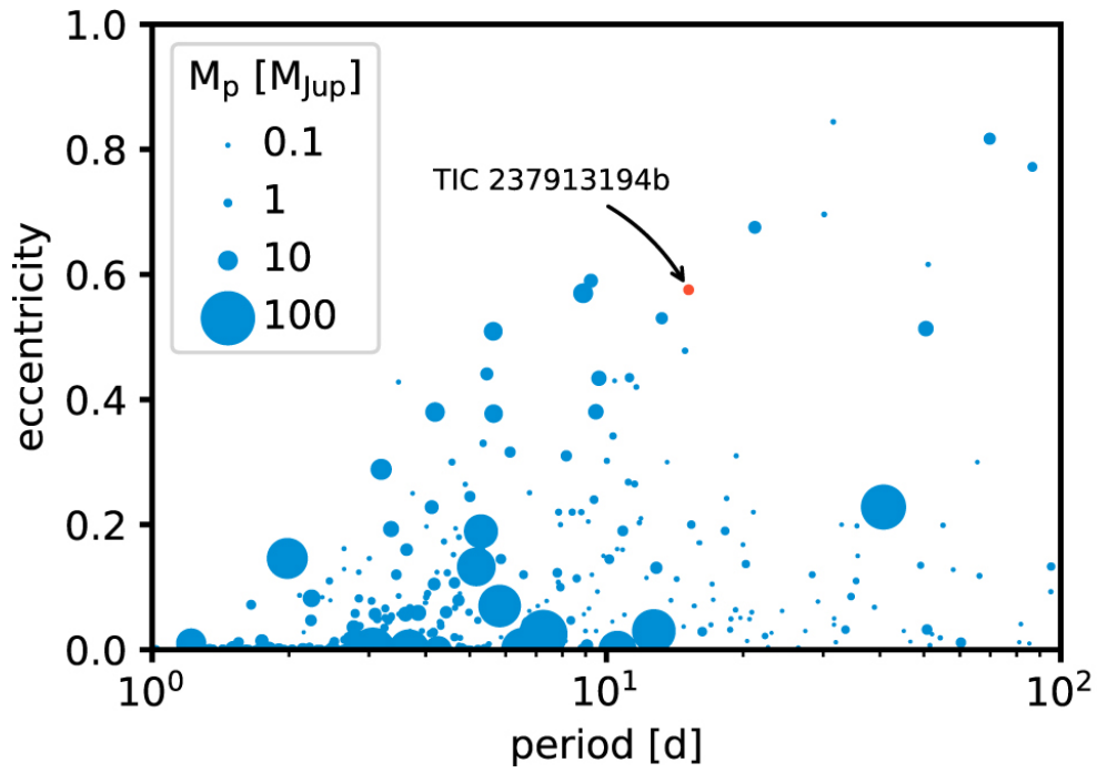
Figure 7. from A Highly Eccentric Warm Jupiter Orbiting TIC 237913194 null 2020 AJ 160 275 doi:10.3847/1538-3881/abbe03 http://dx.doi.org/10.3847/1538-3881/abbe03 © 2020. The American Astronomical Society. All rights reserved.
