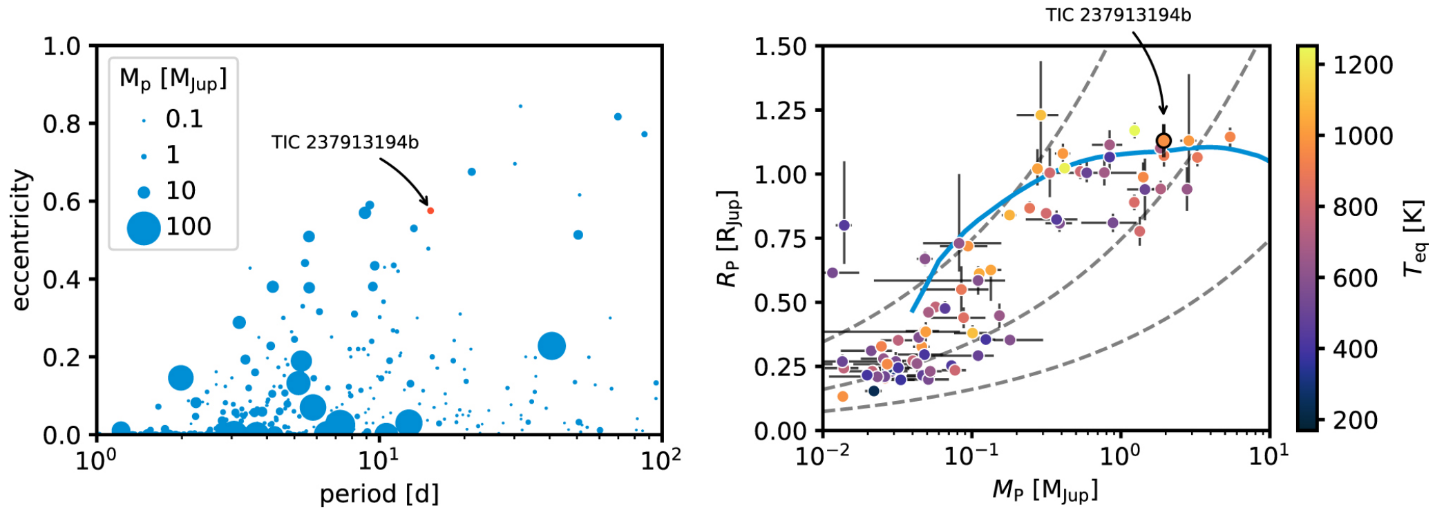
Figure 7. from A Highly Eccentric Warm Jupiter Orbiting TIC 237913194 null 2020 AJ 160 275 doi:10.3847/1538-3881/abbe03 https://dx.doi.org/10.3847/1538-3881/abbe03 © 2020. The American Astronomical Society. All rights reserved.
