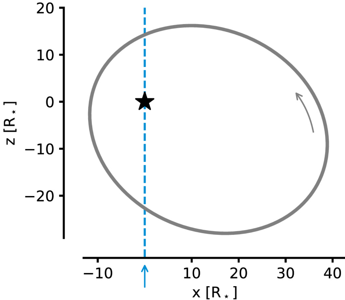
Figure 6. from A Highly Eccentric Warm Jupiter Orbiting TIC 237913194 null 2020 AJ 160 275 doi:10.3847/1538-3881/abbe03 http://dx.doi.org/10.3847/1538-3881/abbe03 © 2020. The American Astronomical Society. All rights reserved.
