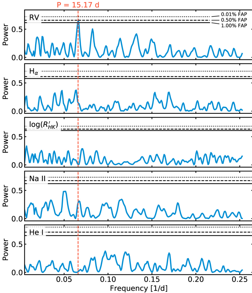
Figure 3. from A Highly Eccentric Warm Jupiter Orbiting TIC 237913194 null 2020 AJ 160 275 doi:10.3847/1538-3881/abbe03 http://dx.doi.org/10.3847/1538-3881/abbe03 © 2020. The American Astronomical Society. All rights reserved.
