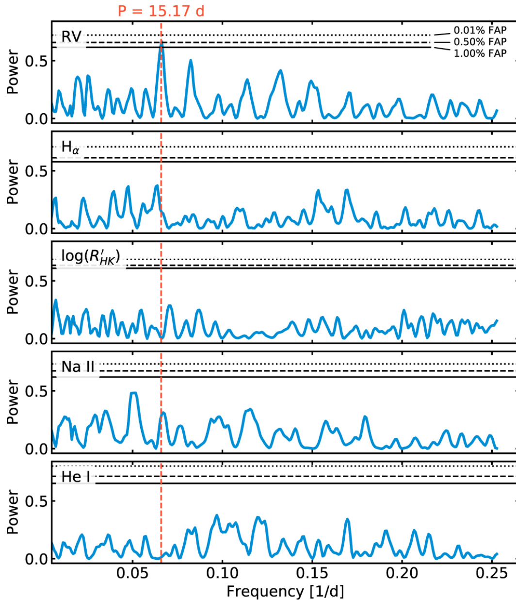
Figure 3. from A Highly Eccentric Warm Jupiter Orbiting TIC 237913194 null 2020 AJ 160 275 doi:10.3847/1538-3881/abbe03 https://dx.doi.org/10.3847/1538-3881/abbe03 © 2020. The American Astronomical Society. All rights reserved.
