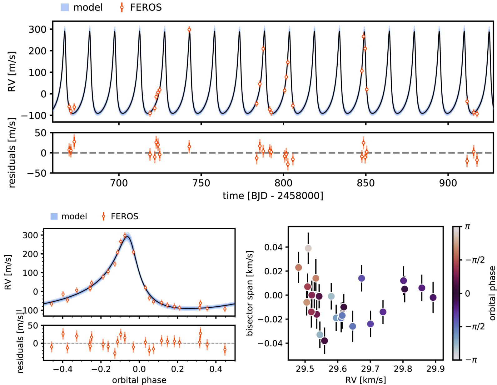
Figure 2. from A Highly Eccentric Warm Jupiter Orbiting TIC 237913194 null 2020 AJ 160 275 doi:10.3847/1538-3881/abbe03 https://dx.doi.org/10.3847/1538-3881/abbe03 © 2020. The American Astronomical Society. All rights reserved.
