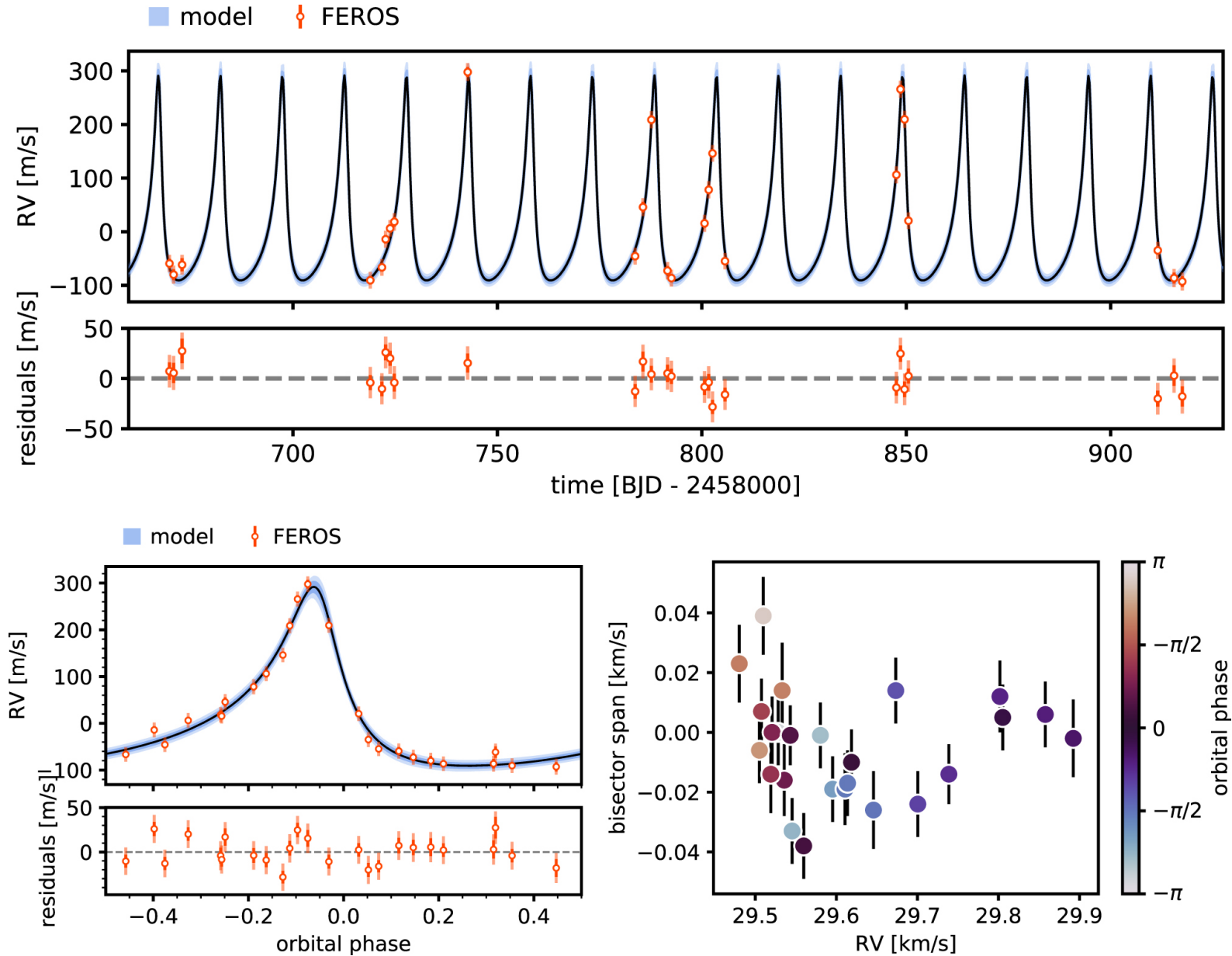
Figure 2. from A Highly Eccentric Warm Jupiter Orbiting TIC 237913194 null 2020 AJ 160 275 doi:10.3847/1538-3881/abbe03 http://dx.doi.org/10.3847/1538-3881/abbe03 © 2020. The American Astronomical Society. All rights reserved.
