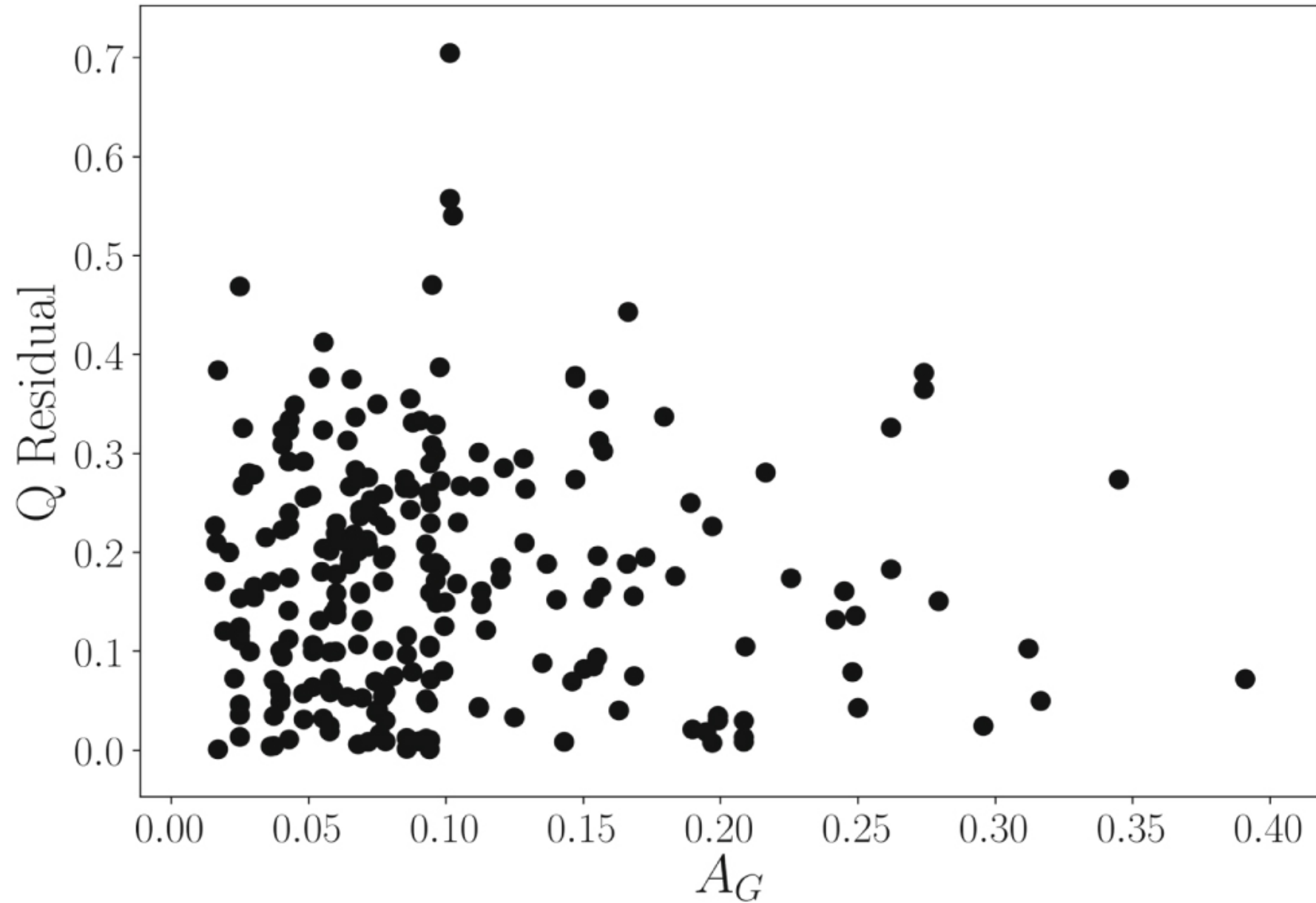
Figure 10. from Estimating the Ages of FGK Dwarf Stars through the Use of GALEX FUV Magnitudes null 2020 AJ 160 217 doi:10.3847/1538-3881/abb77d https://dx.doi.org/10.3847/1538-3881/abb77d © 2020. The American Astronomical Society. All rights reserved.
