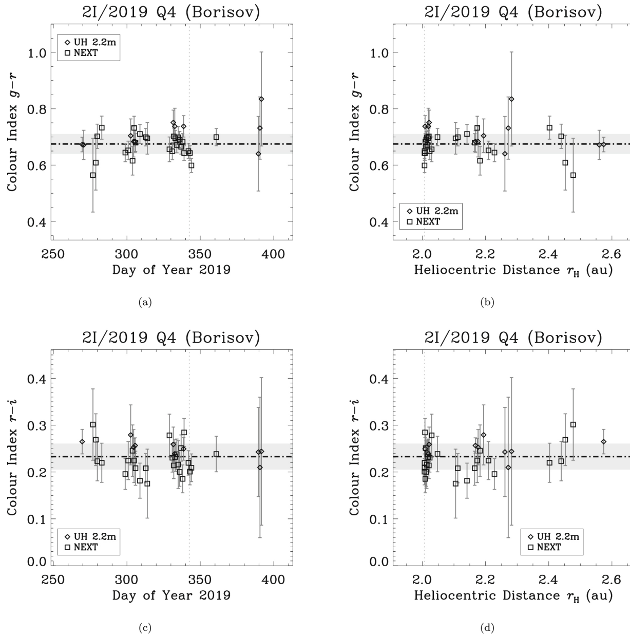
Figure 6. from Physical Characterization of Interstellar Comet 2I/2019 Q4 (Borisov) null 2020 AJ 160 92 doi:10.3847/1538-3881/ab9df8 https://dx.doi.org/10.3847/1538-3881/ab9df8 © 2020. The American Astronomical Society. All rights reserved.
