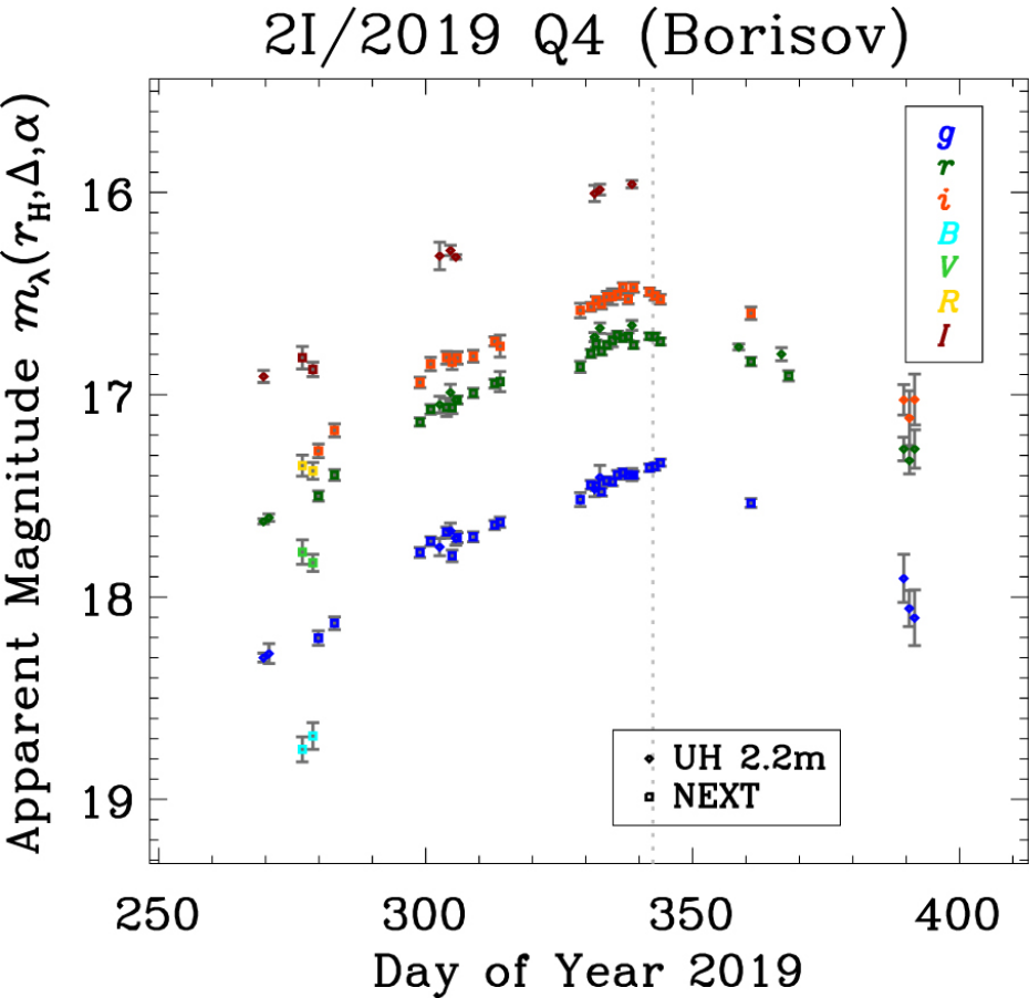
Figure 4. from Physical Characterization of Interstellar Comet 2I/2019 Q4 (Borisov) null 2020 AJ 160 92 doi:10.3847/1538-3881/ab9df8 https://dx.doi.org/10.3847/1538-3881/ab9df8 © 2020. The American Astronomical Society. All rights reserved.
