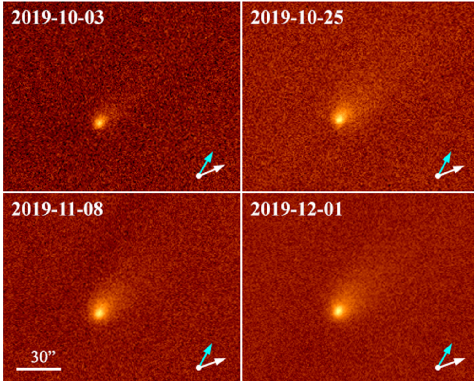
Figure 3. from Physical Characterization of Interstellar Comet 2I/2019 Q4 (Borisov) null 2020 AJ 160 92 doi:10.3847/1538-3881/ab9df8 https://dx.doi.org/10.3847/1538-3881/ab9df8 © 2020. The American Astronomical Society. All rights reserved.
