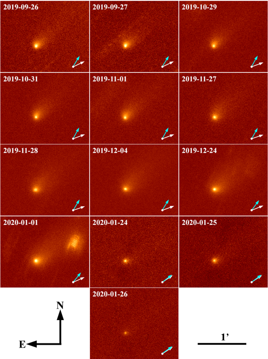
Figure 2. from Physical Characterization of Interstellar Comet 2I/2019 Q4 (Borisov) null 2020 AJ 160 92 doi:10.3847/1538-3881/ab9df8 https://dx.doi.org/10.3847/1538-3881/ab9df8 © 2020. The American Astronomical Society. All rights reserved.
