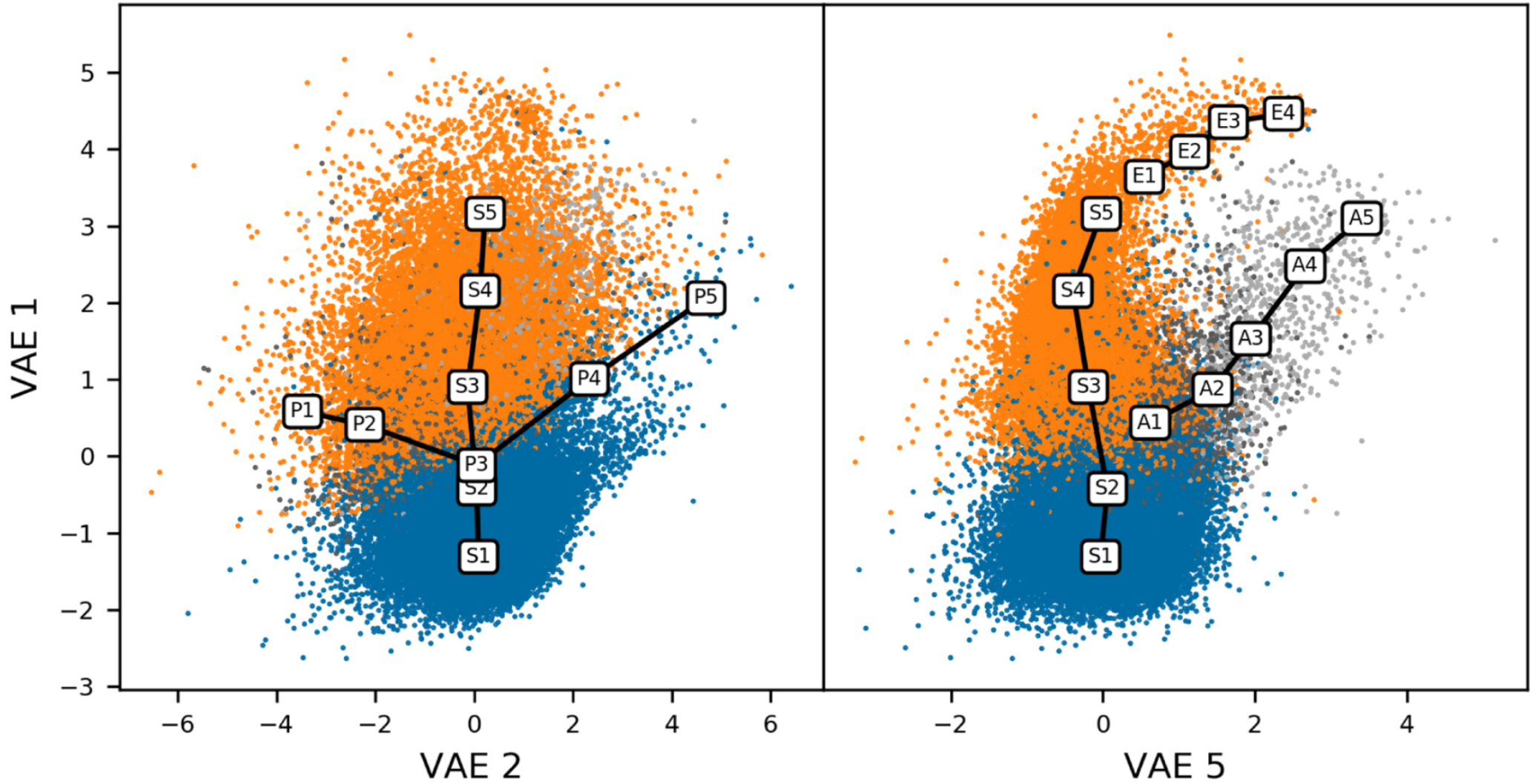
Figure 9. from Dimensionality Reduction of SDSS Spectra with Variational Autoencoders null 2020 AJ 160 45 doi:10.3847/1538-3881/ab9644 http://dx.doi.org/10.3847/1538-3881/ab9644 © 2020. The American Astronomical Society. All rights reserved.
