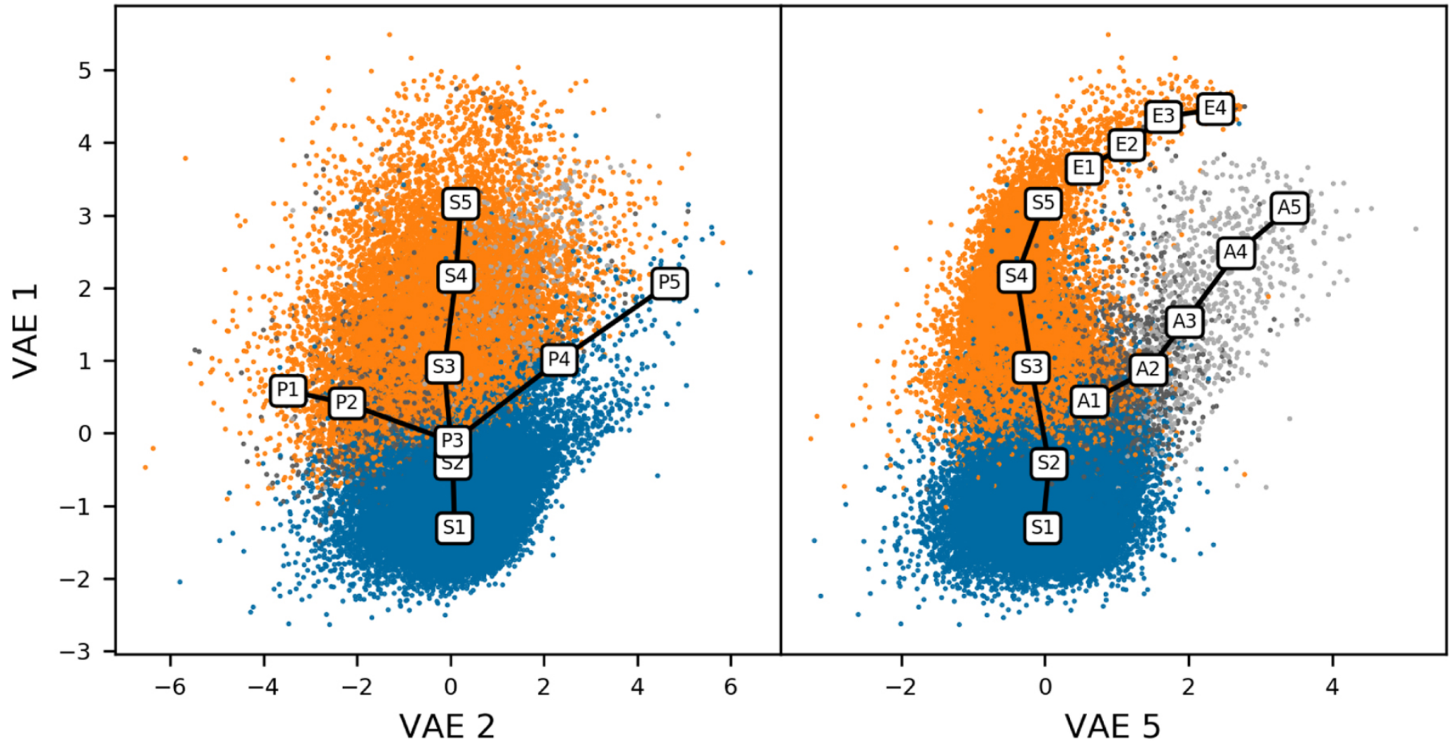
Figure 9. from Dimensionality Reduction of SDSS Spectra with Variational Autoencoders null 2020 AJ 160 45 doi:10.3847/1538-3881/ab9644 https://dx.doi.org/10.3847/1538-3881/ab9644 © 2020. The American Astronomical Society. All rights reserved.
