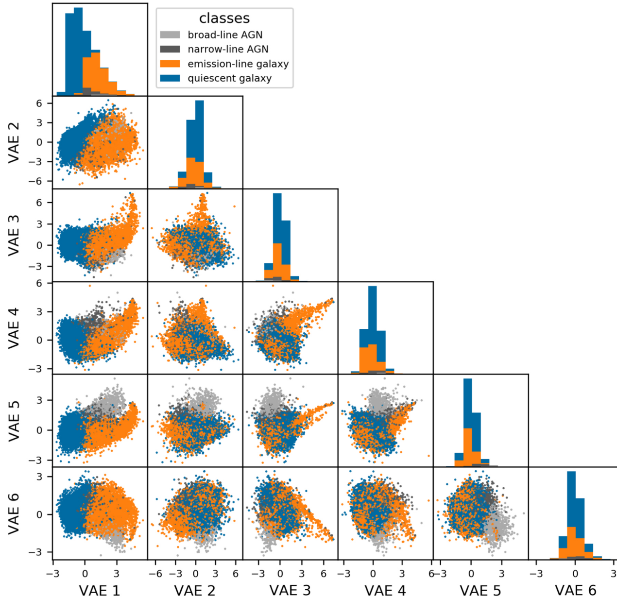
Figure 8. from Dimensionality Reduction of SDSS Spectra with Variational Autoencoders null 2020 AJ 160 45 doi:10.3847/1538-3881/ab9644 https://dx.doi.org/10.3847/1538-3881/ab9644 © 2020. The American Astronomical Society. All rights reserved.
