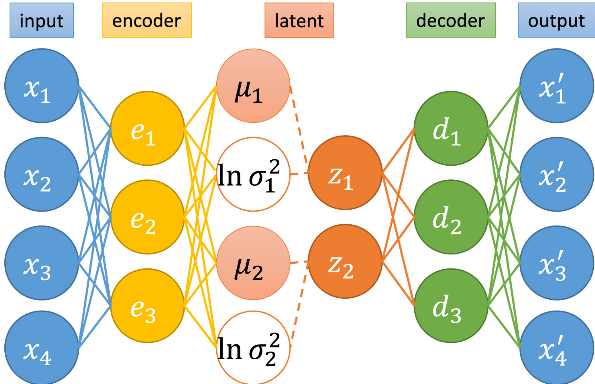
Figure 2. from Dimensionality Reduction of SDSS Spectra with Variational Autoencoders null 2020 AJ 160 45 doi:10.3847/1538-3881/ab9644 https://dx.doi.org/10.3847/1538-3881/ab9644 © 2020. The American Astronomical Society. All rights reserved.
