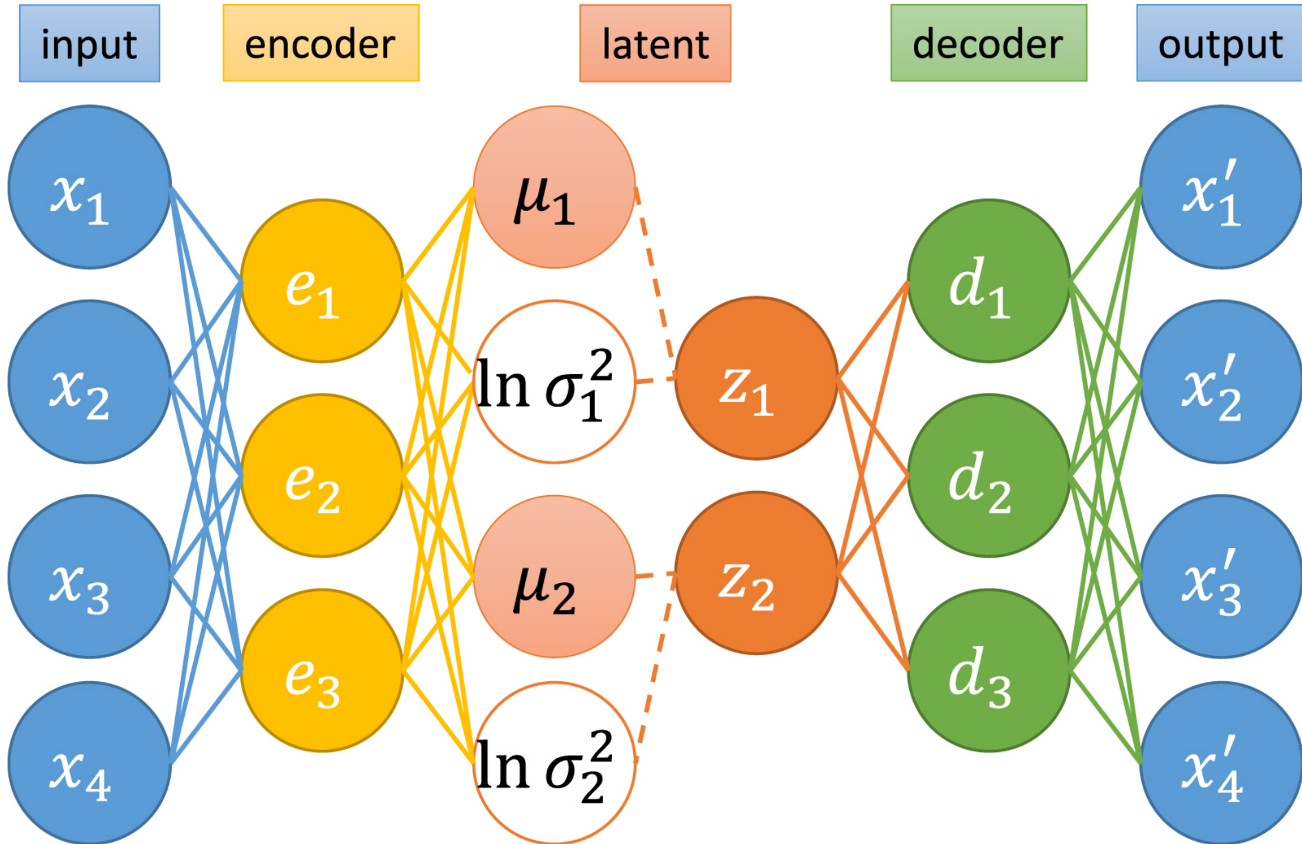
Figure 2. from Dimensionality Reduction of SDSS Spectra with Variational Autoencoders null 2020 AJ 160 45 doi:10.3847/1538-3881/ab9644 http://dx.doi.org/10.3847/1538-3881/ab9644 © 2020. The American Astronomical Society. All rights reserved.
