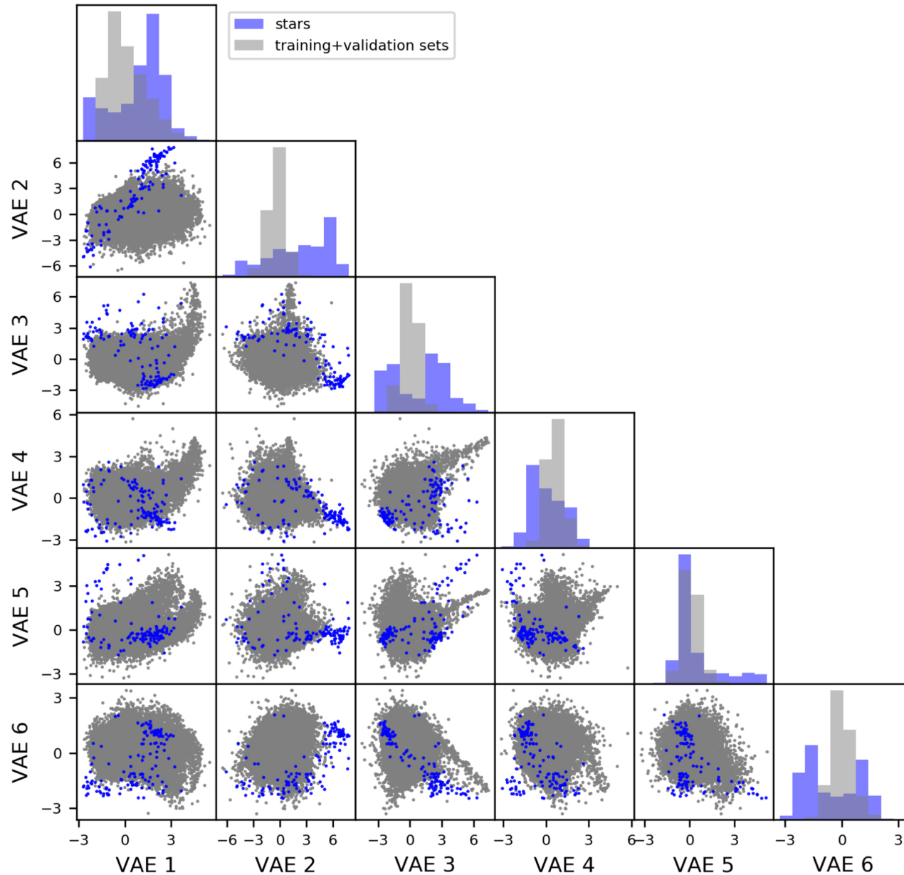
Figure 16. from Dimensionality Reduction of SDSS Spectra with Variational Autoencoders null 2020 AJ 160 45 doi:10.3847/1538-3881/ab9644 https://dx.doi.org/10.3847/1538-3881/ab9644 © 2020. The American Astronomical Society. All rights reserved.
