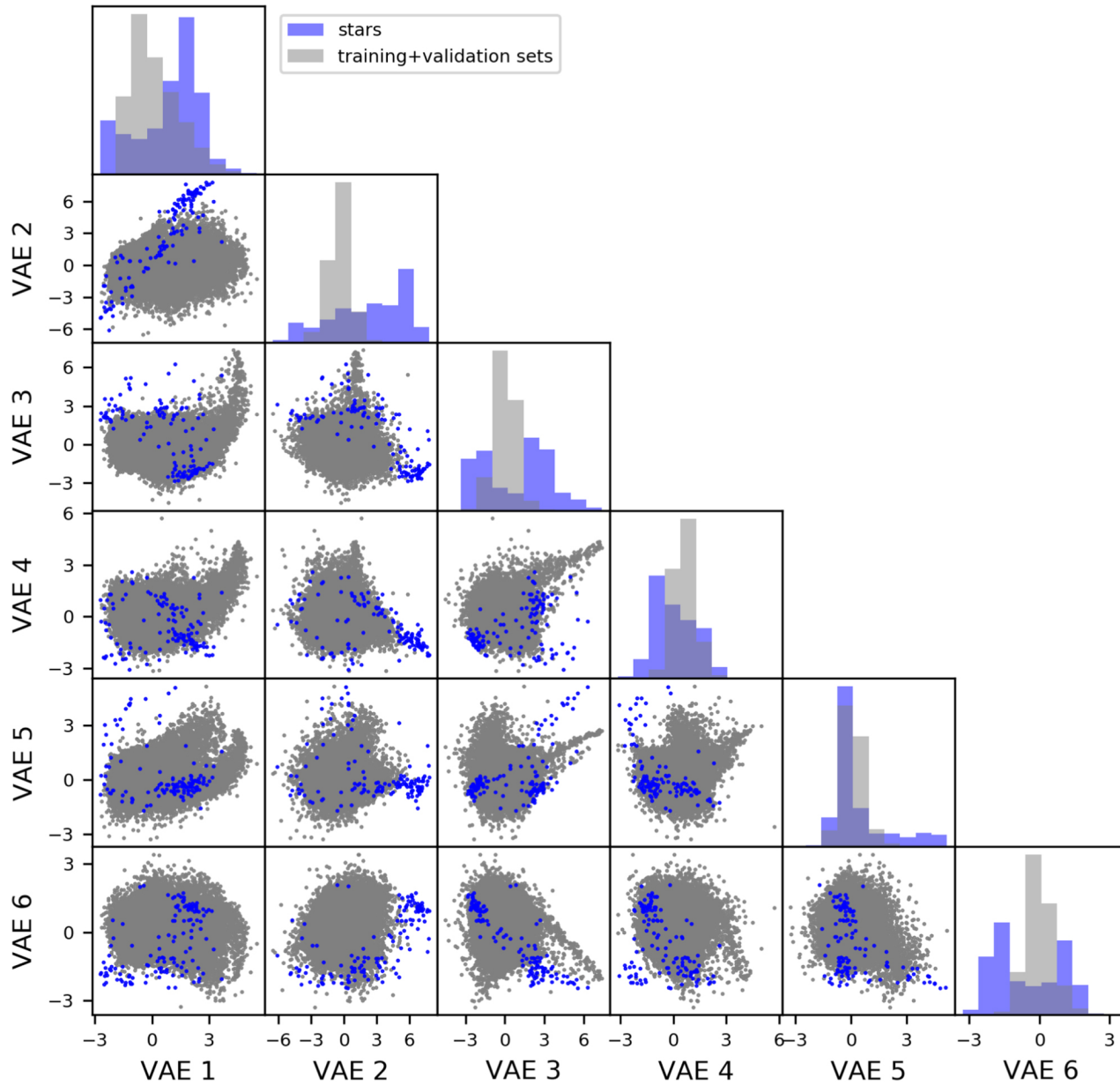
Figure 16. from Dimensionality Reduction of SDSS Spectra with Variational Autoencoders null 2020 AJ 160 45 doi:10.3847/1538-3881/ab9644 http://dx.doi.org/10.3847/1538-3881/ab9644 © 2020. The American Astronomical Society. All rights reserved.
