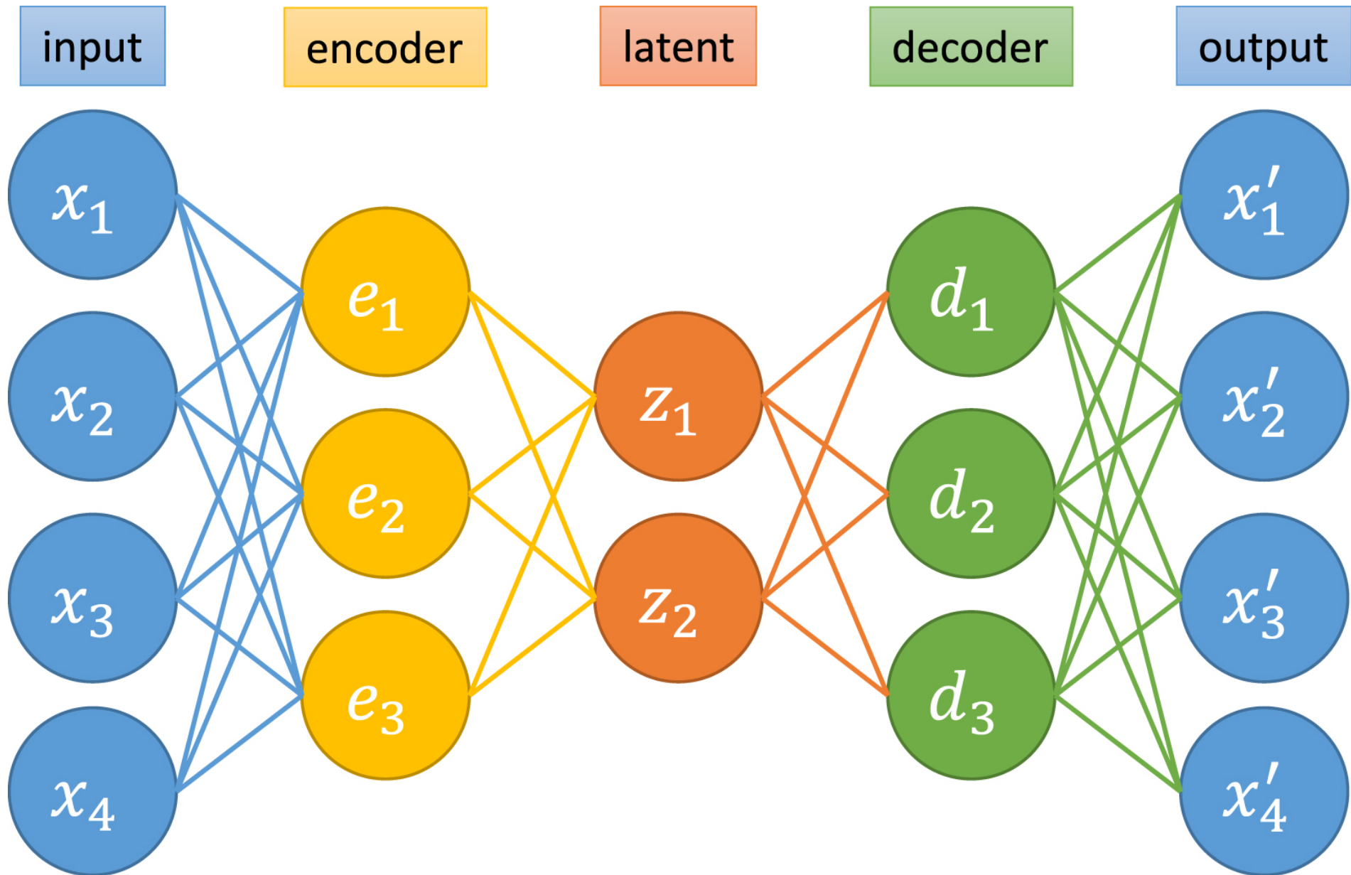
Figure 1. from Dimensionality Reduction of SDSS Spectra with Variational Autoencoders null 2020 AJ 160 45 doi:10.3847/1538-3881/ab9644 http://dx.doi.org/10.3847/1538-3881/ab9644 © 2020. The American Astronomical Society. All rights reserved.
