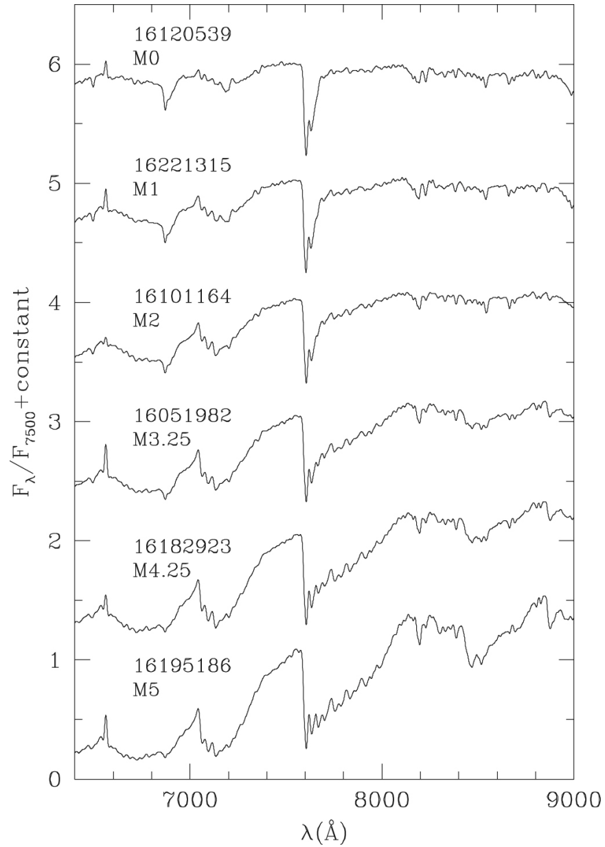
Figure 7. from Refining the Census of the Upper Scorpius Association with Gaia null 2020 AJ 160 44 doi:10.3847/1538-3881/ab9599 https://dx.doi.org/10.3847/1538-3881/ab9599 © 2020. The American Astronomical Society. All rights reserved.
