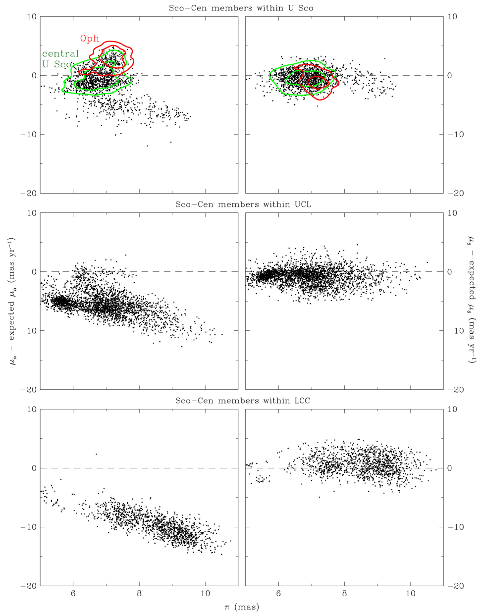
Figure 6. from Refining the Census of the Upper Scorpius Association with Gaia null 2020 AJ 160 44 doi:10.3847/1538-3881/ab9599 https://dx.doi.org/10.3847/1538-3881/ab9599 © 2020. The American Astronomical Society. All rights reserved.
